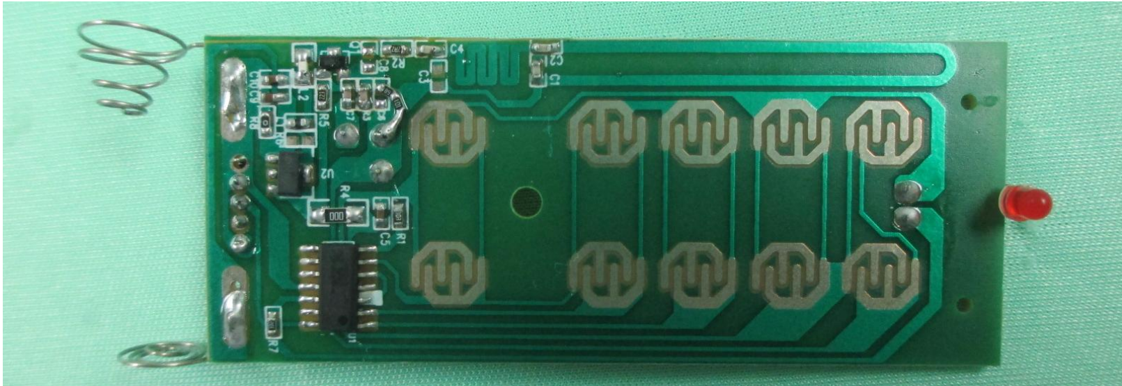
INNER CIRCUIT BOTTOM VIEW
