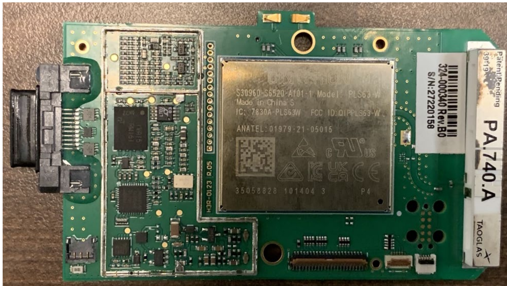
Exhibit: Internal Photos (Top PCBA with EMI Shield Removed) (FCC ID: ZIMH41L; EUT IC ID: 9647A-H41L)
