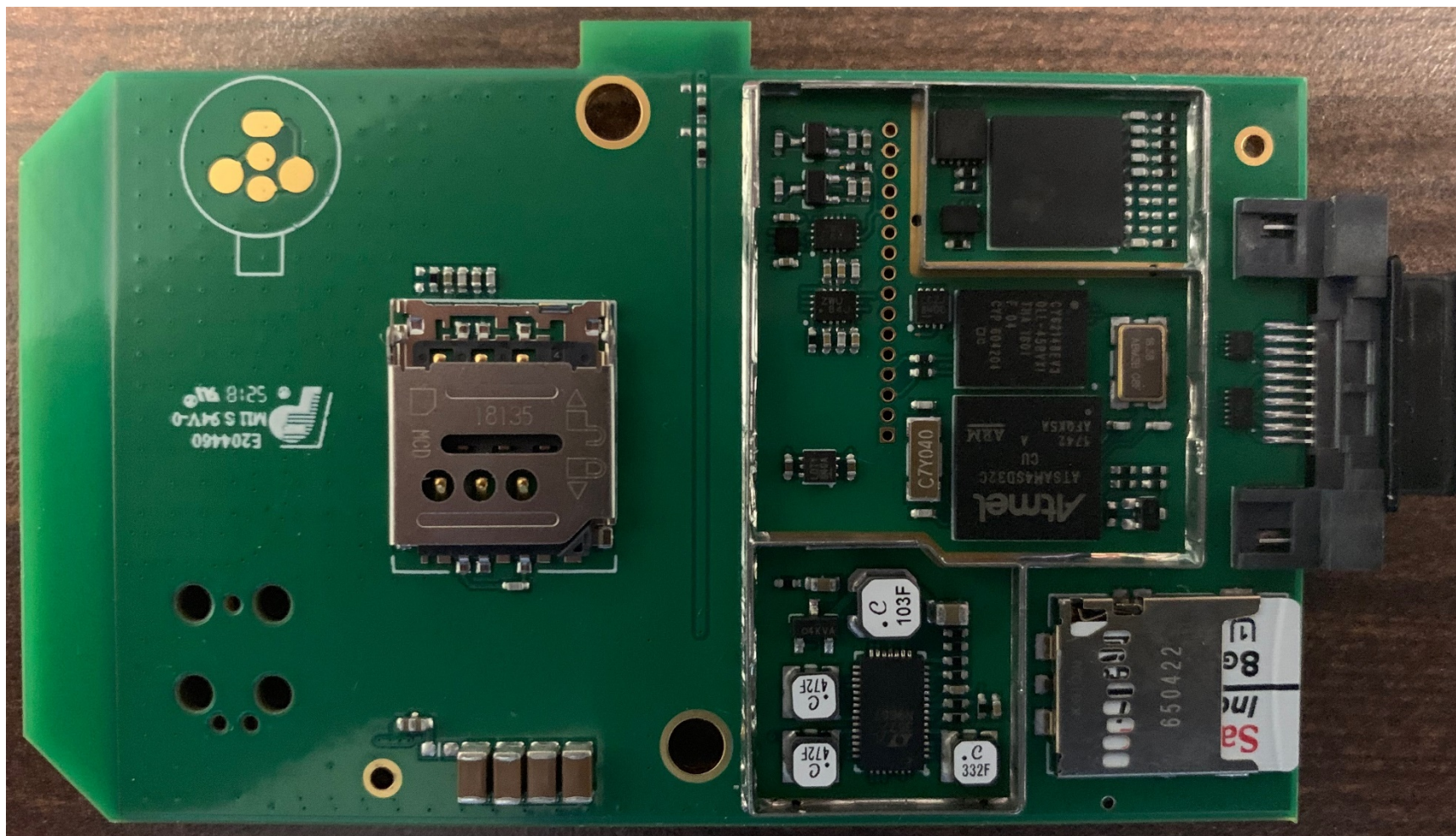
Exhibit: Internal Photos (Bottom PCBA with EMI Shield Removed) (FCC ID: ZIMH41L; EUT IC ID: 9647A-H41L)
