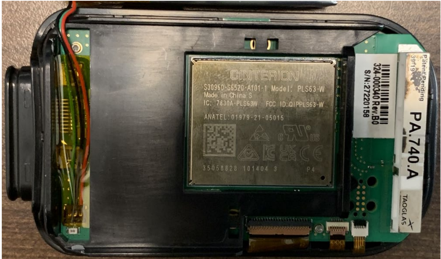
Exhibit: Internal Photos (Interior with Battery Removed) (FCC ID: ZIMH41L; EUT IC ID: 9647A-H41L)
