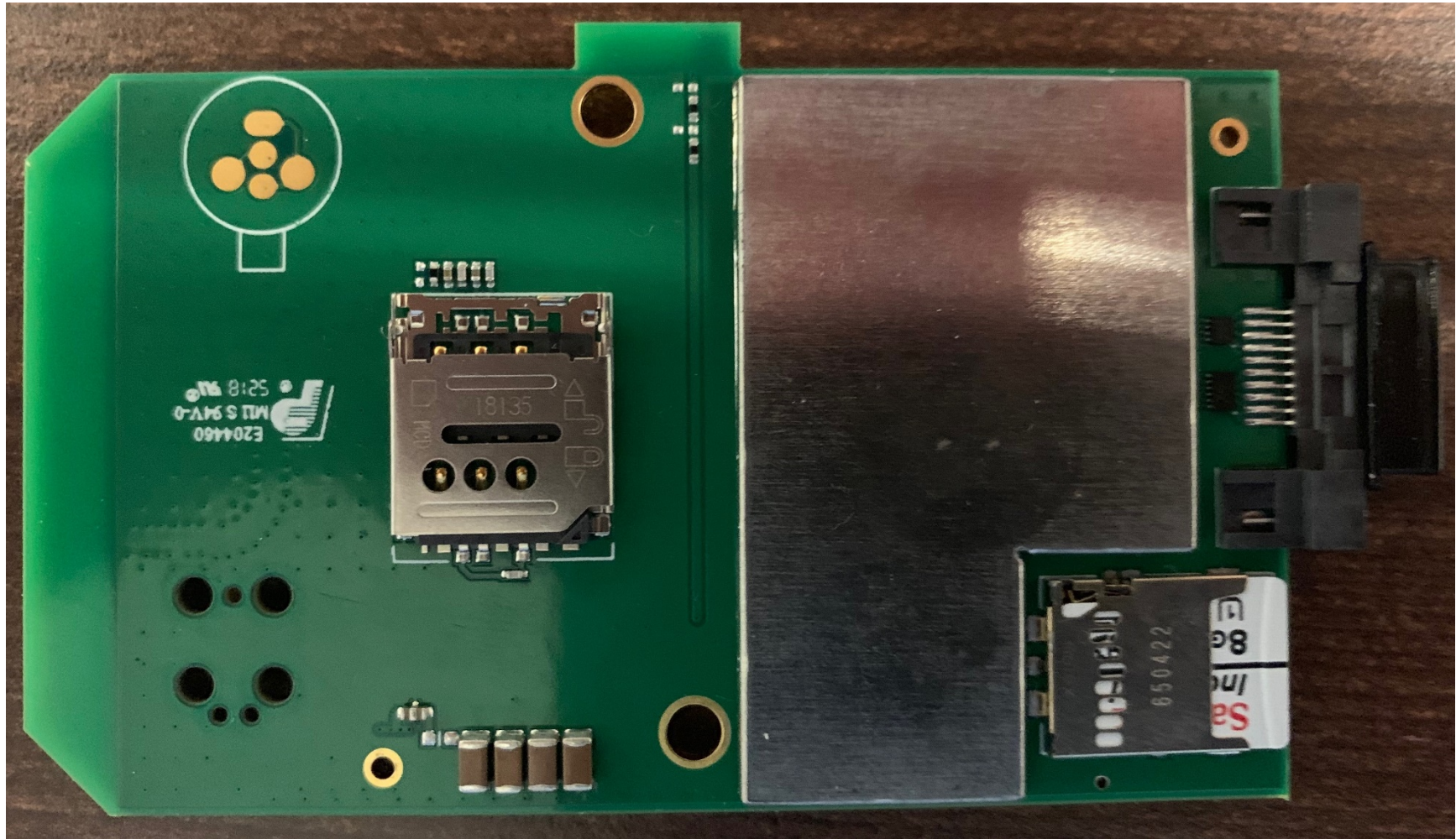
Exhibit: Internal Photos (Bottom PCBA with EMI Shield) (FCC ID: ZIMH41L; EUT IC ID: 9647A-H41L)
