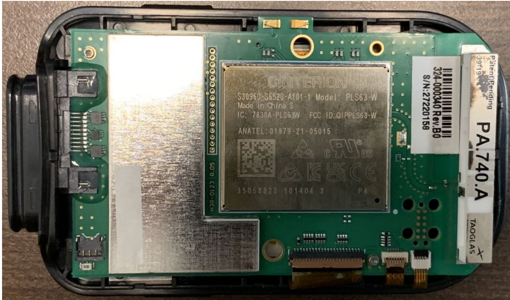
Exhibit: Internal Photos (Interior with Battery Holder / Antenna Removed) (FCC ID: ZIMH41L; EUT IC ID: 9647A-H41L)
