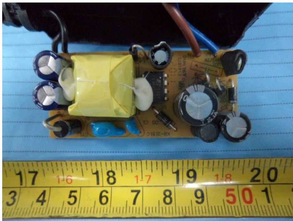
EUT – Adapter Main Board Top View
