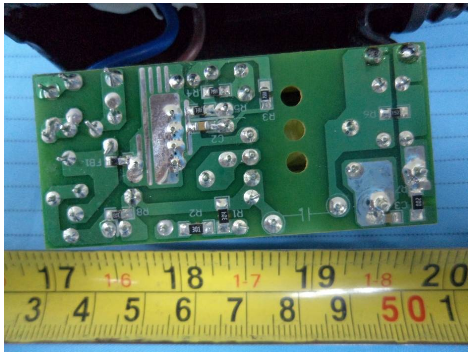
EUT – Adapter Main Board Bottom View
