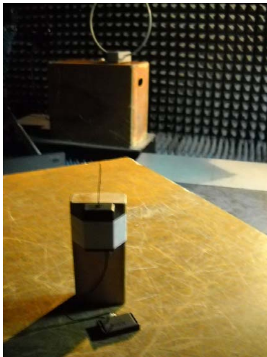
Photograph No.1 Setup for spurious emission measurements in the anechoic chamber below 30 MHz
