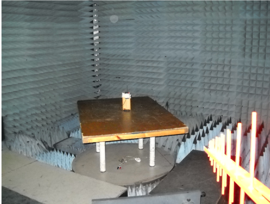
Photograph No.2 Setup for radiated emission measurements in the anechoic chamber from 30 to 1000 MHz
