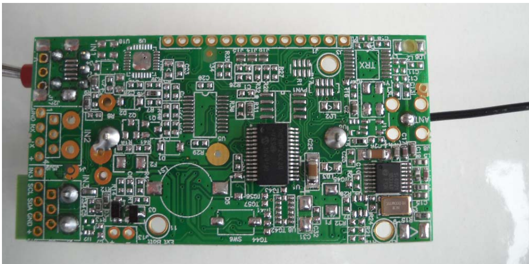
Photograph No.3 Component side of the main/RF PCB
