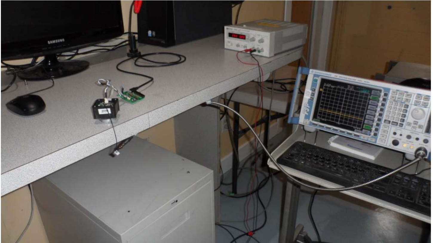
Figure E23.1 – Setup Photo – Conducted Measurements – Host 1
