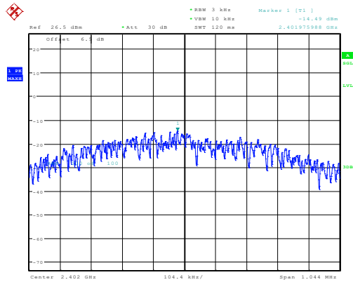
Low -14.49dBm/3kHz
