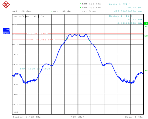
Low 0.696MHz
