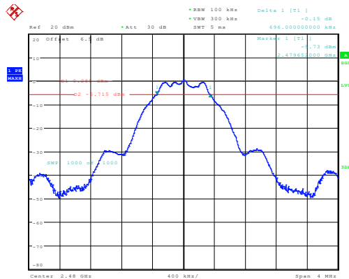
High 0.696MHz
