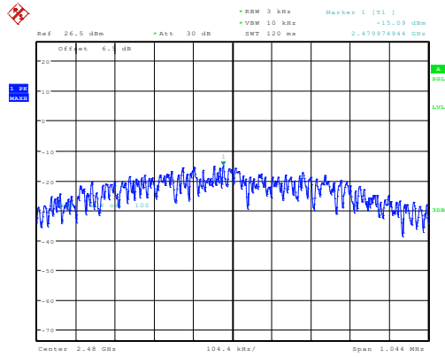
High -15.09dBm/3kHz
