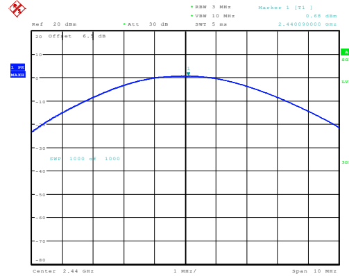
Middle 0.68dBm
