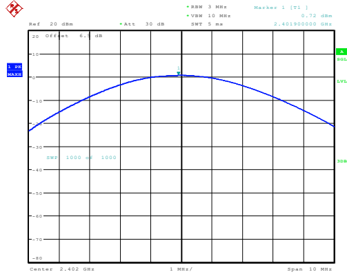
Low 0.72dBm
