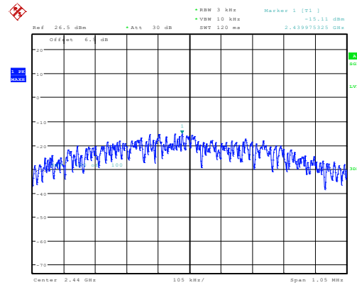
Middle -15.11dBm/3kHz
