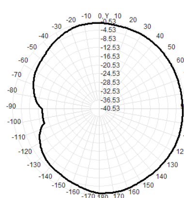
Total(H-XY), Max= -2.05dBi, CirD=17.22
