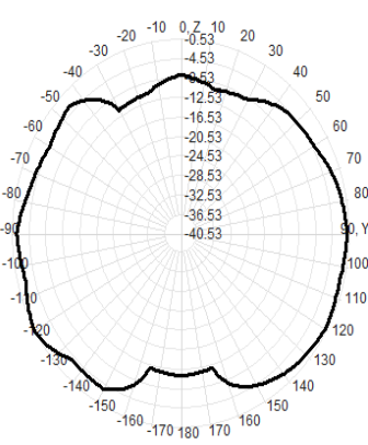
2480.0MHz Total(E2-YZ), Max= -1.61dBi
