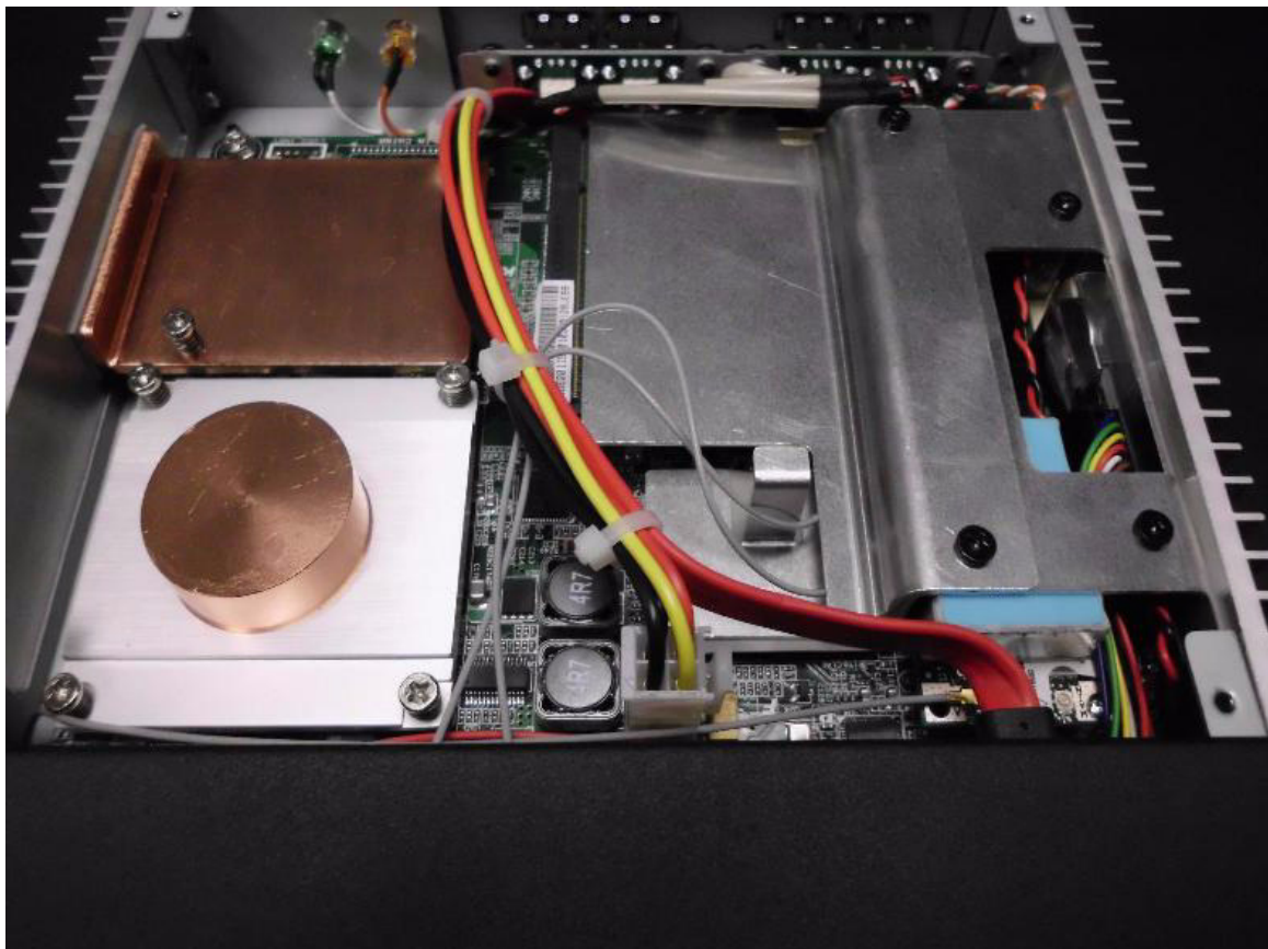
Camera interior with heatsinks installed
