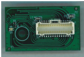
Imager Interface circuit board top view
