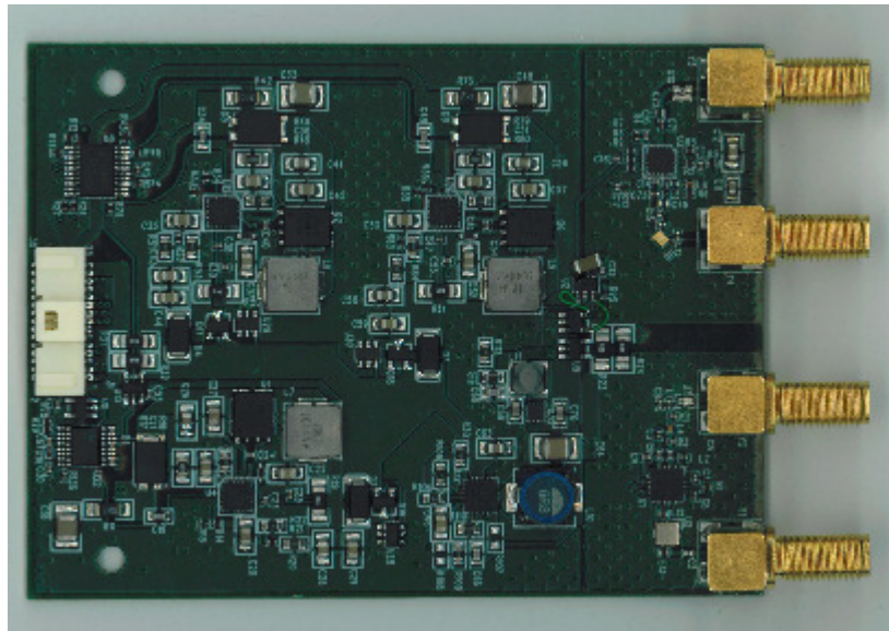
PA/Solar circuit board top view
