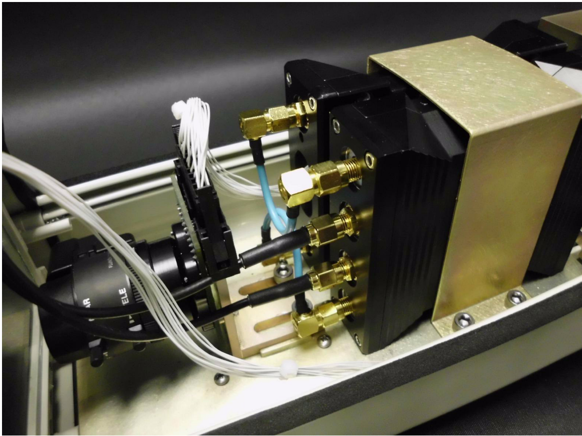
Camera interior RF connector detail
