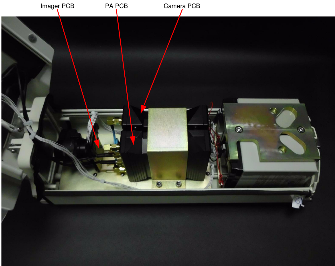
Camera interior base
