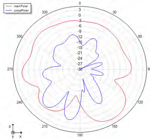
Phi=0 freq=2446MHz
