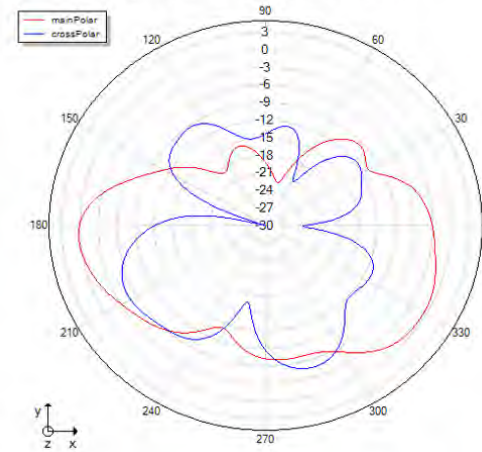
Theta=90 freq=2446MHz
