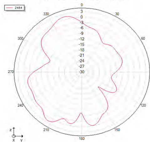
Phi=90 freq=2454MHz
