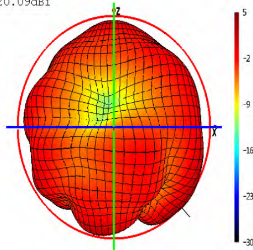
Phi=0 freq=2454MHz
