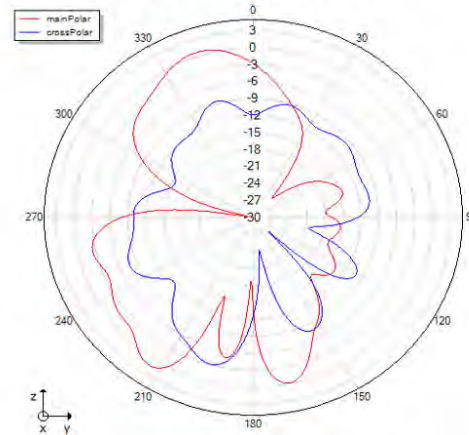
Phi=90 freq=2480MHz
