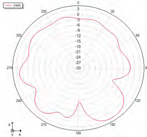
Phi=0 freq=2480MHz
