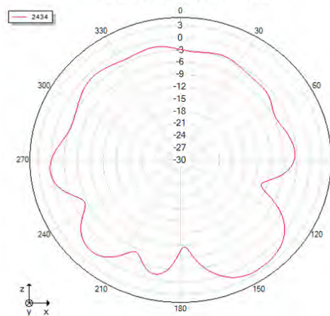
Phi=0 freq=2434MHz
