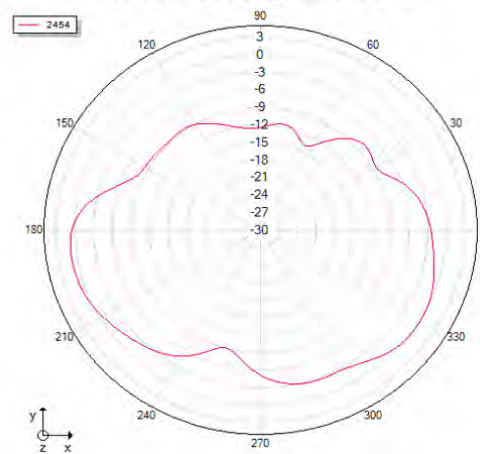
Theta=90 freq=2454MHz
