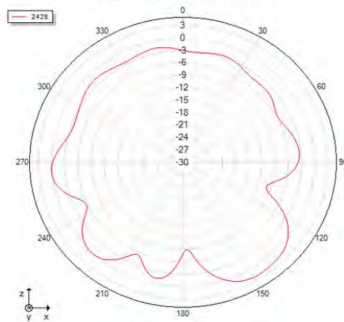
Phi=0 freq=2428MHz
