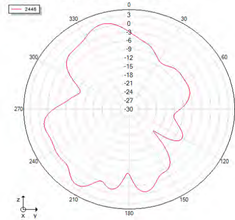
Phi=90 freq=2446MHz
