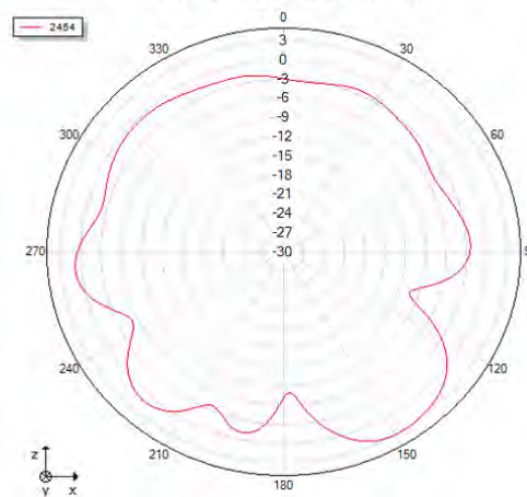
Phi=0 freq=2454MHz
