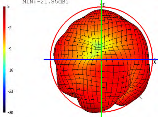
Phi=0 freq=2428MHz
