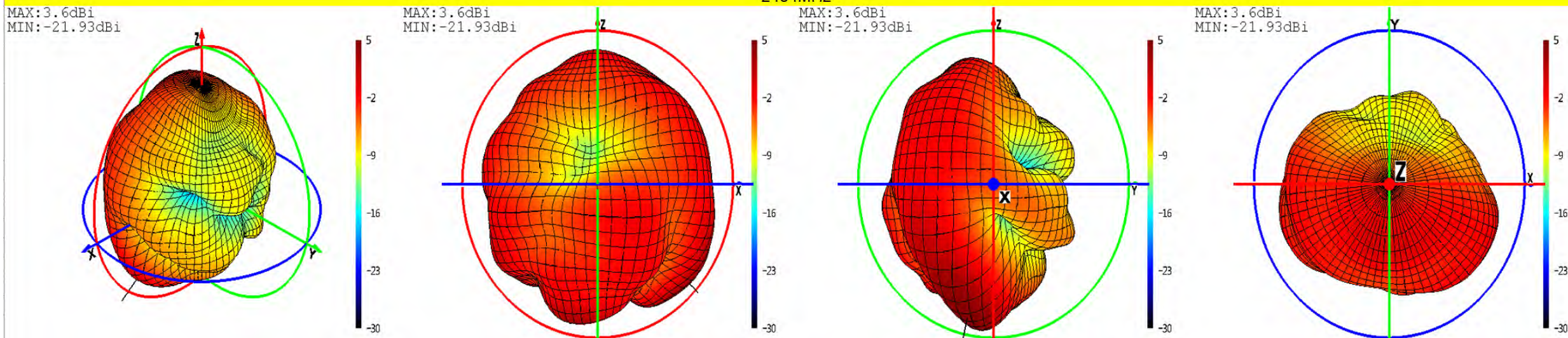
Phi=0 freq=2434MHz
