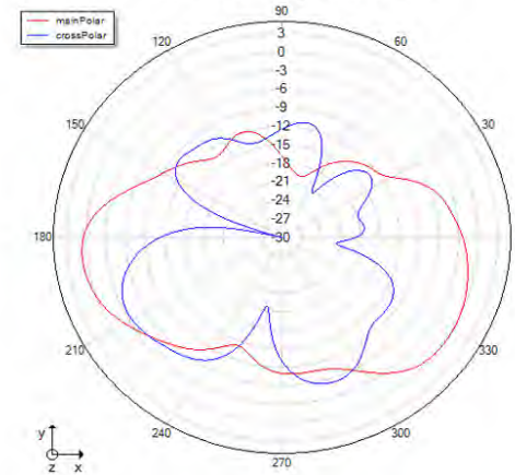
Theta=90 freq=2480MHz
