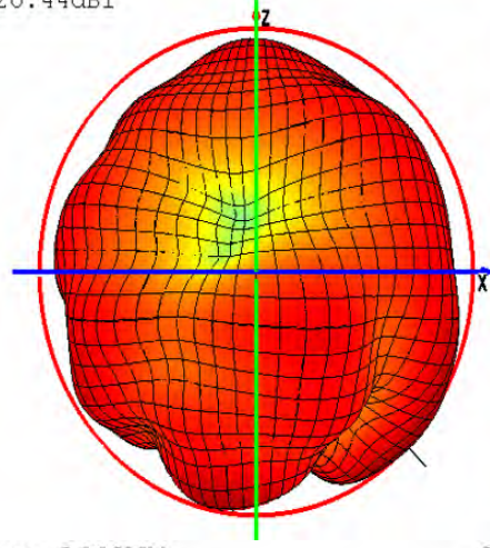
Phi=0 freq=2446MHz
