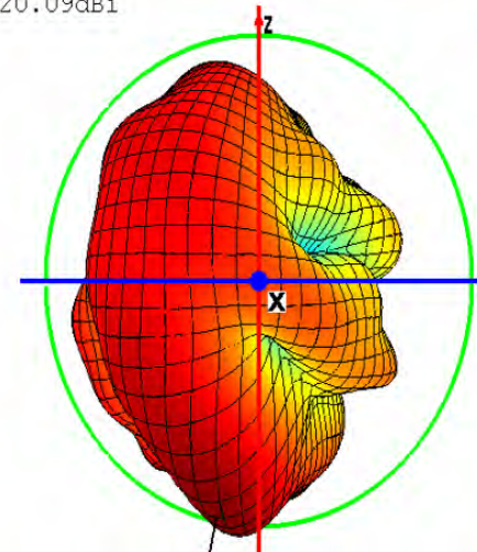
Theta=90 freq=2454MHz
