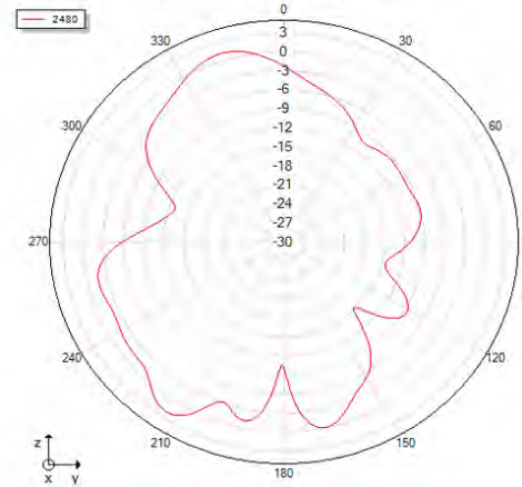
Phi=90 freq=2480MHz
