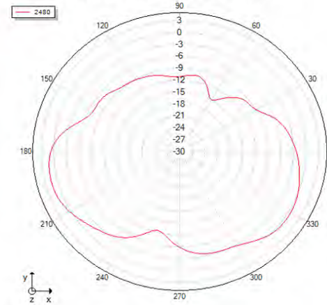
Theta=90 freq=2480MHz
