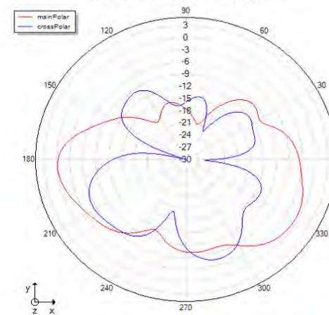
Theta=90 freq=2434MHz
