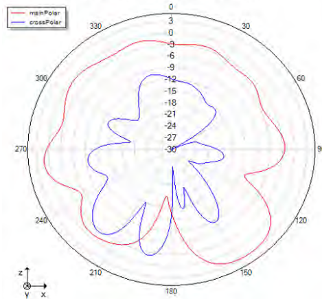
Phi=0 freq=2480MHz
