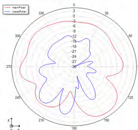
Phi=0 freq=2454MHz
