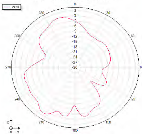
Phi=90 freq=2428MHz
