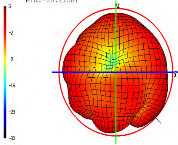
Phi=0 freq=2480MHz
