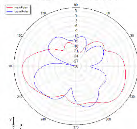
Theta=90 freq=2454MHz
