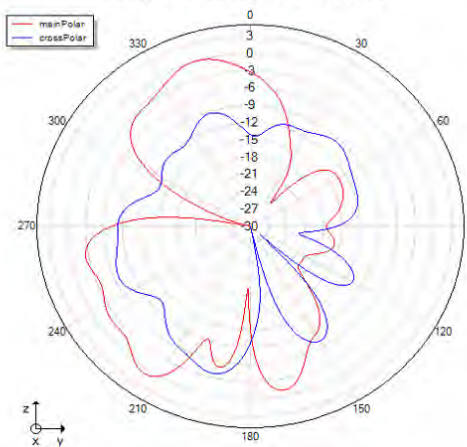
Phi=90 freq=2434MHz
