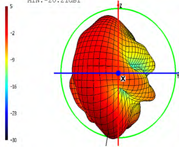
Phi=90 freq=2480MHz
