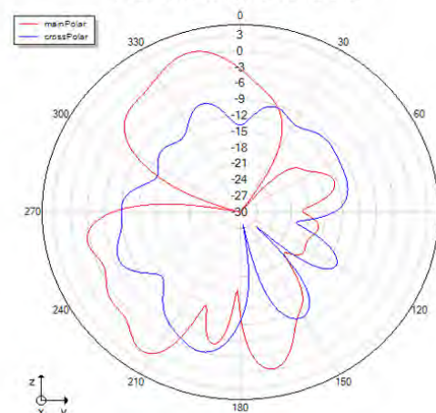
Phi=90 freq=2454MHz
