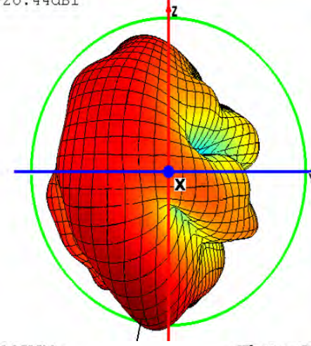
Phi=90 freq=2446MHz
