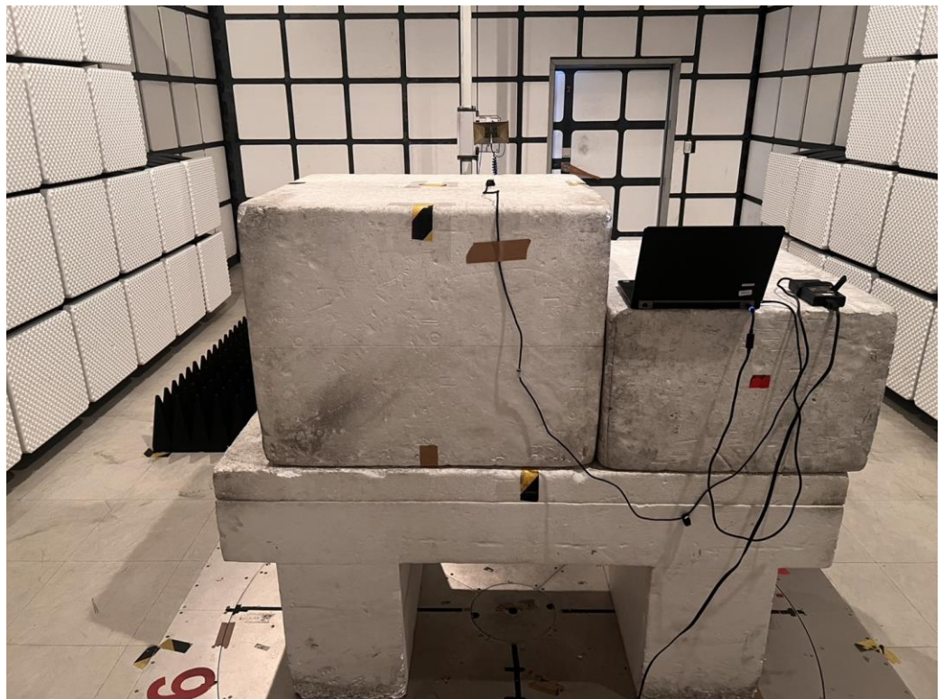
Rear View
