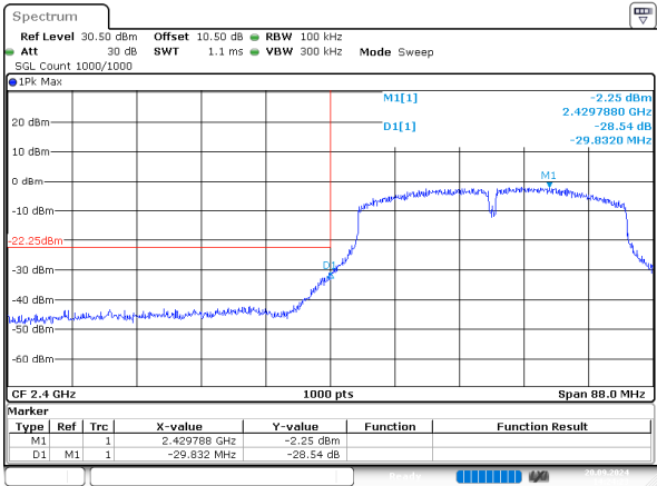
n40_2422MHz_Chain 0
