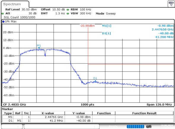
n40_2452MHz_Chain 0
