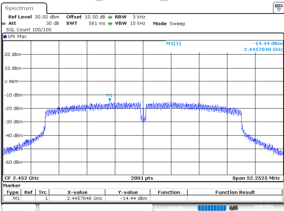
n40_2452MHz_Chain 1
