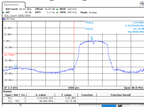
n20_2412MHz_Chain 0
