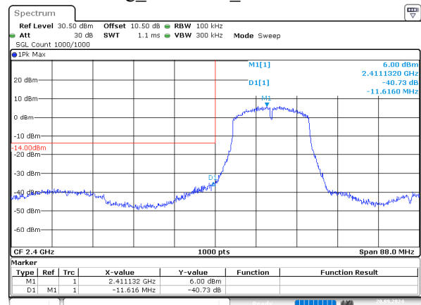
g_2412MHz_Chain 1
