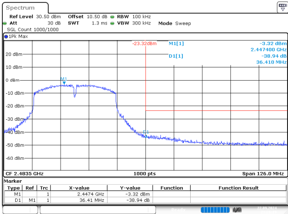
n40_2452MHz_Chain 1
