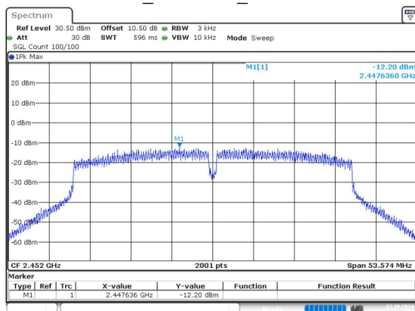
n40_2452MHz_Chain 0
