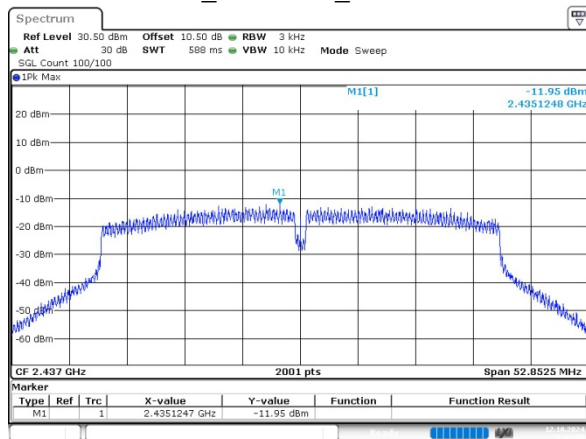
n40_2437MHz_Chain 0
