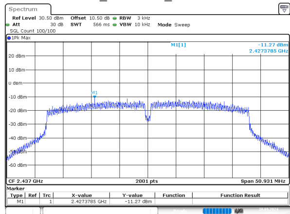
n40_2437MHz_Chain 1
