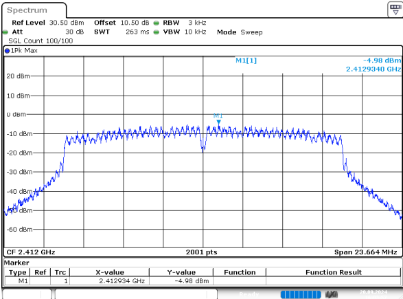
g_2412MHz_Chain 1
