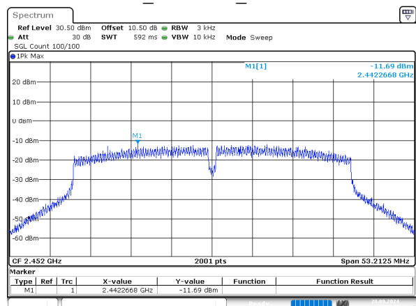
n40_2452MHz_Chain 1
