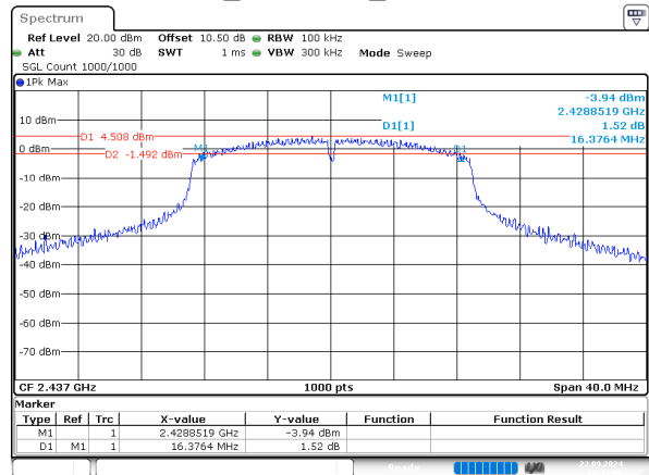
n20_2437MHz_Chain 0
