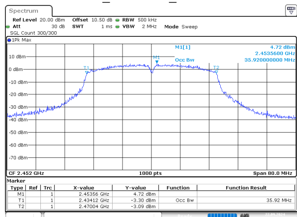
n40_2452MHz_Chain 0
