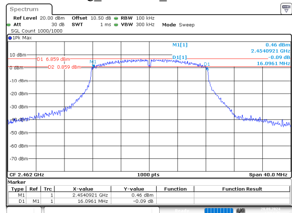
g_2462MHz_Chain 0
