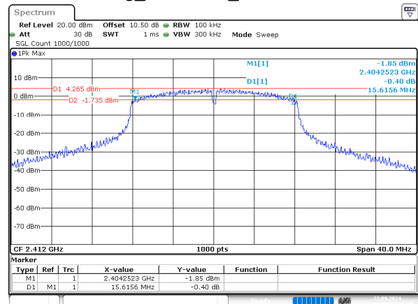
g_2412MHz_Chain 0
