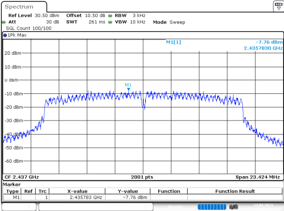
g_2437MHz_Chain 1
