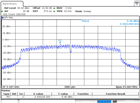
n20_2437MHz_Chain 0
