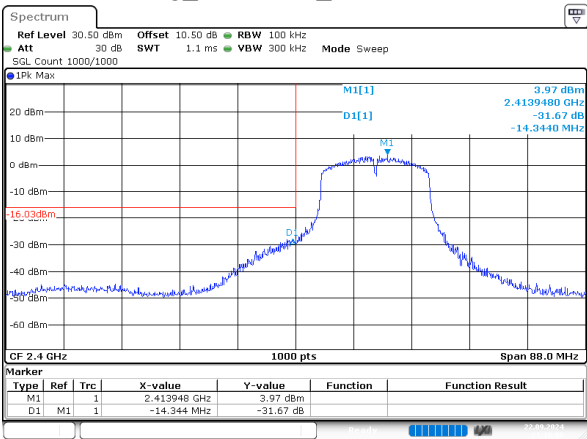
g_2412MHz_Chain 1
