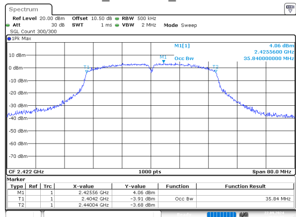
n40_2422MHz_Chain 0
