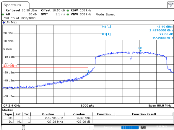
n40_2422MHz_Chain 1
