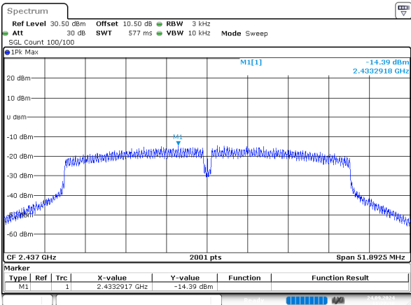
n40_2437MHz_Chain 1
