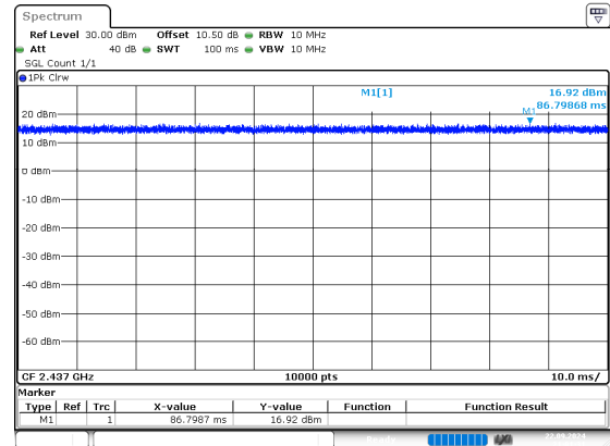
n40_2437MHz_Chain 0
