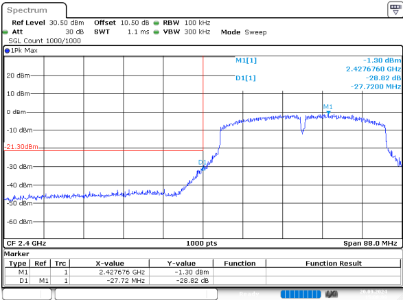
n40_2422MHz_Chain 1
