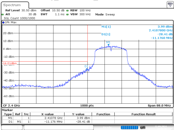
g_2412MHz_Chain 0
