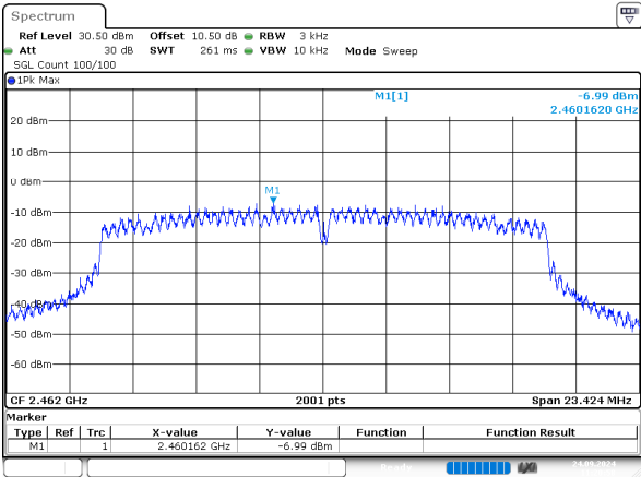
g_2462MHz_Chain 1
