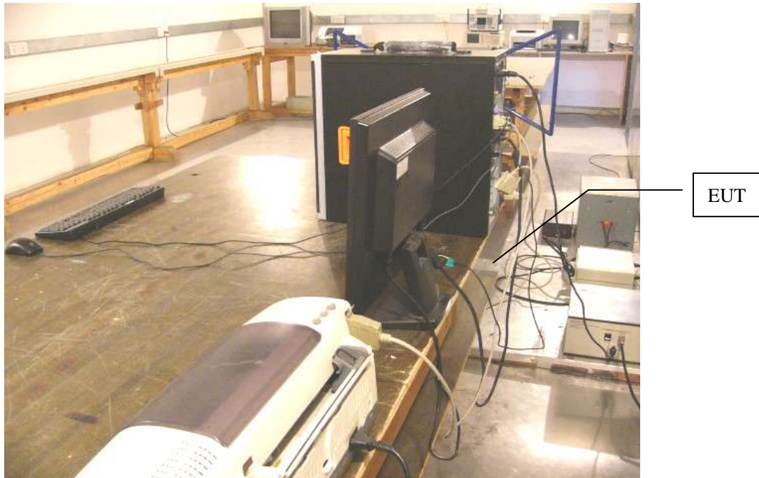
Radiated emission test view
