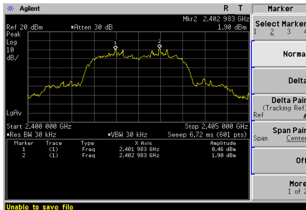
TEST PLOT FOR FREQUENCY SEPARATION ( 3Mbps )
