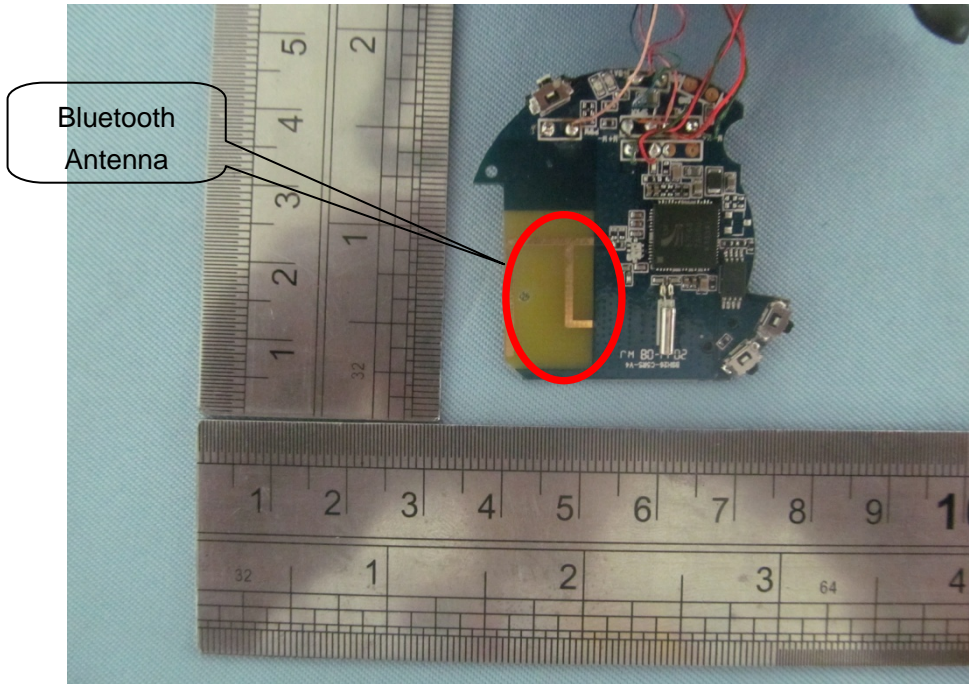
BACK VIEW OF PCB-1
