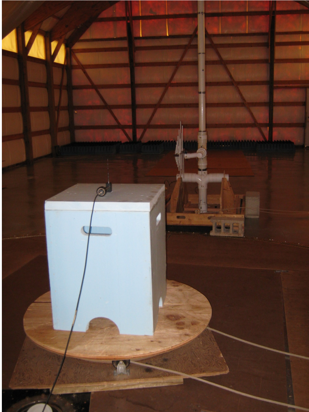
Photo Description: Substitution Measurement Setup – Angle 2
