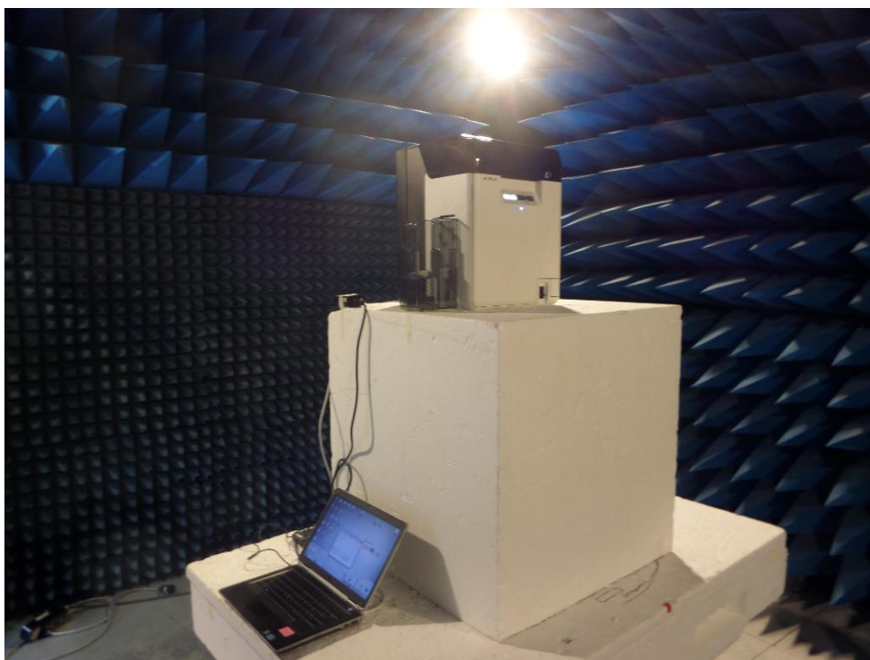
Anechoic room
