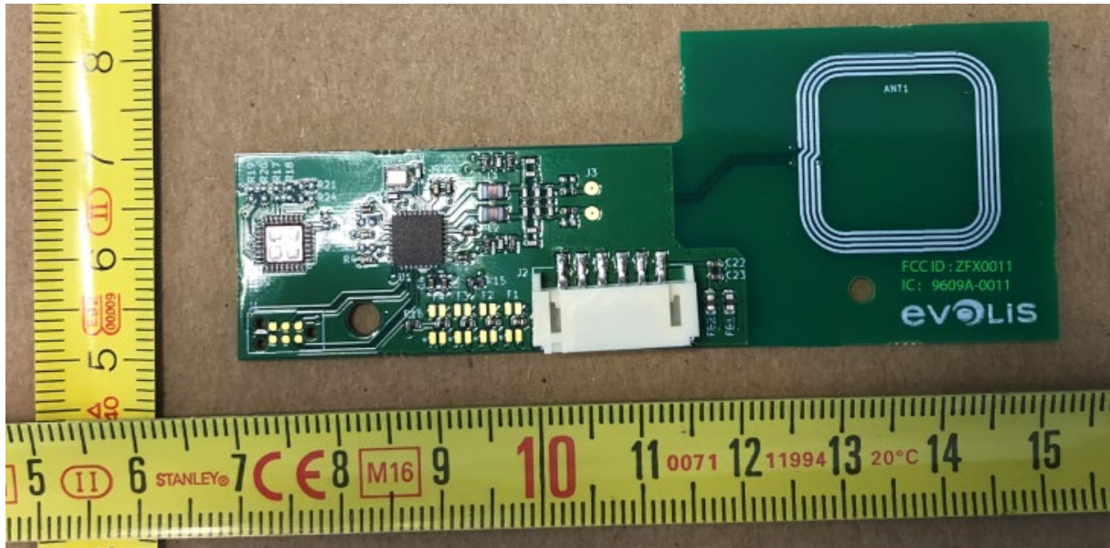
Rear view
