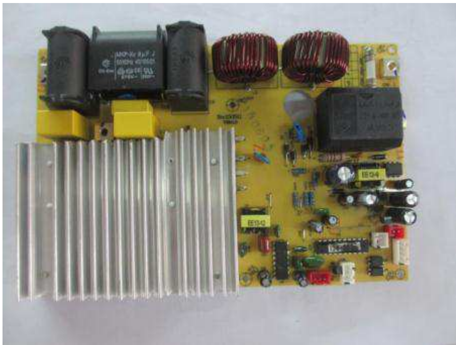
Burner A
