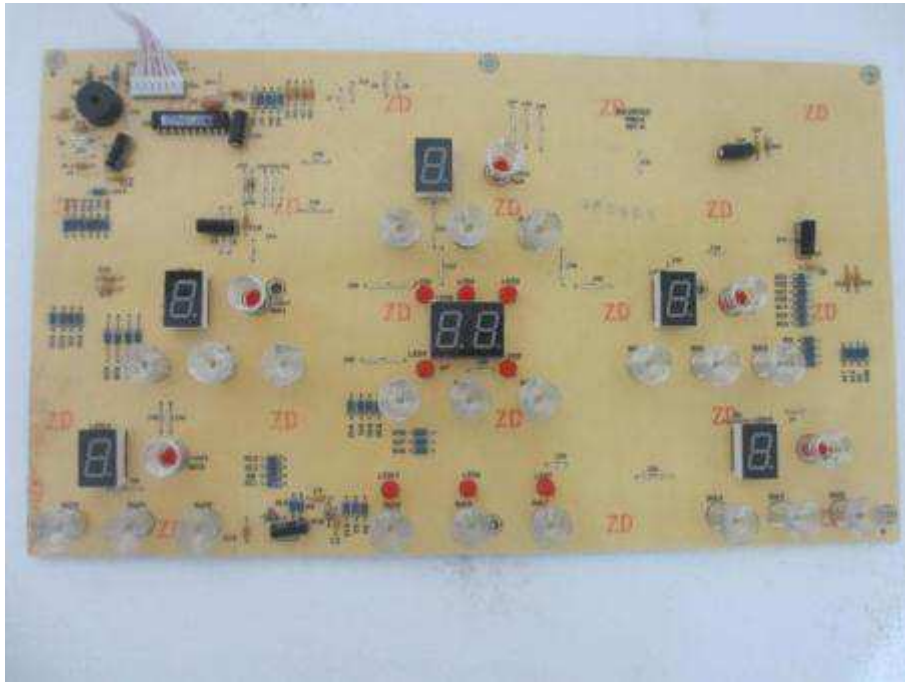
Control PCB:
