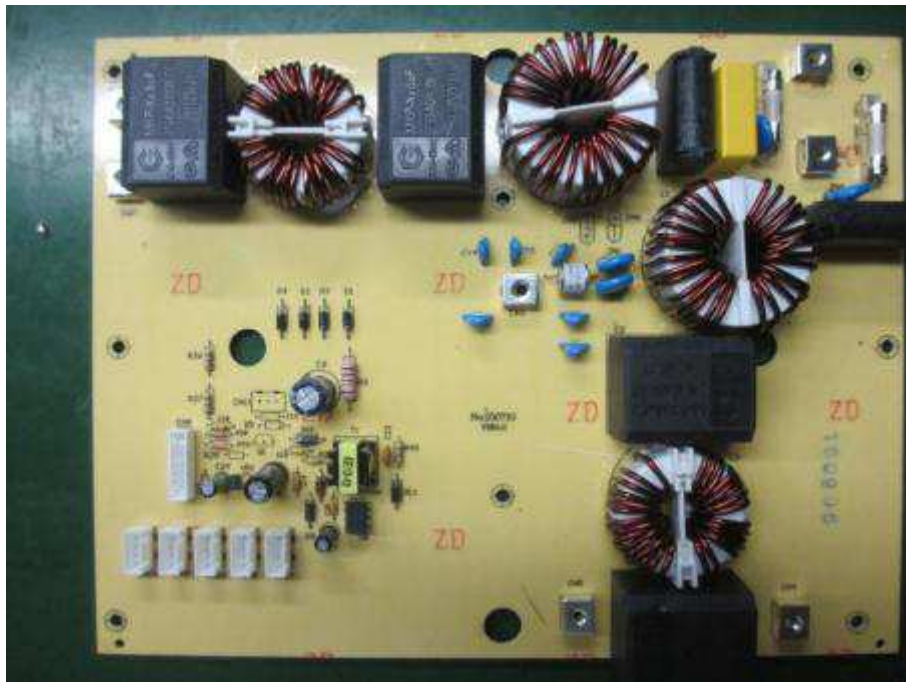
Power PCB:
