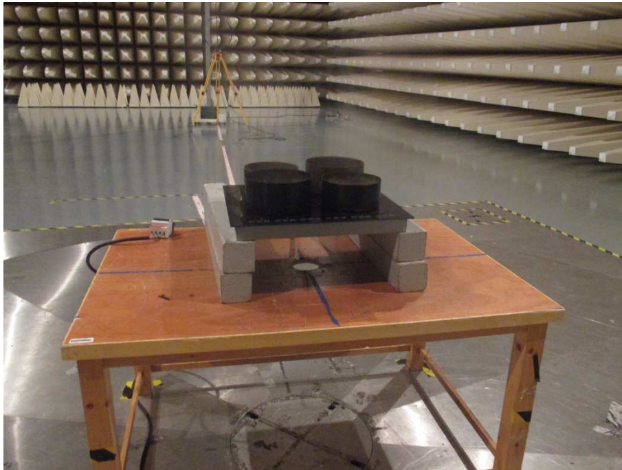
Radiated Emission 9k-30MHz
