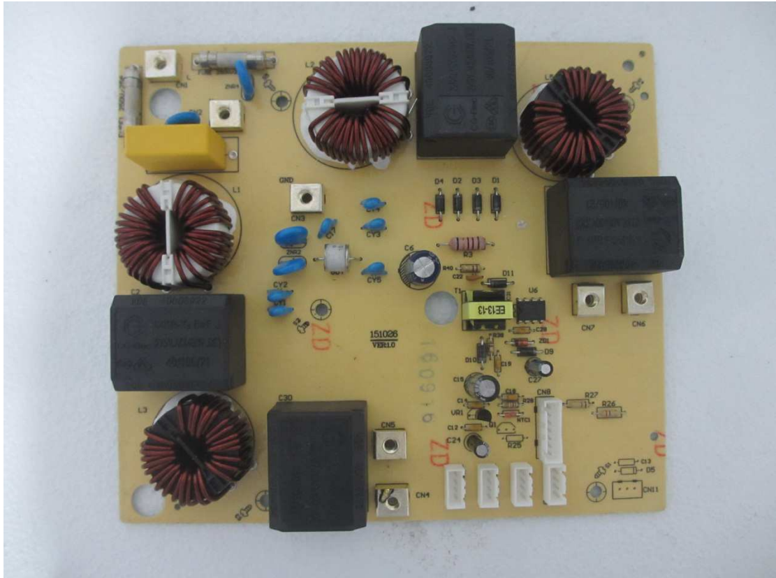
Power PCB:
