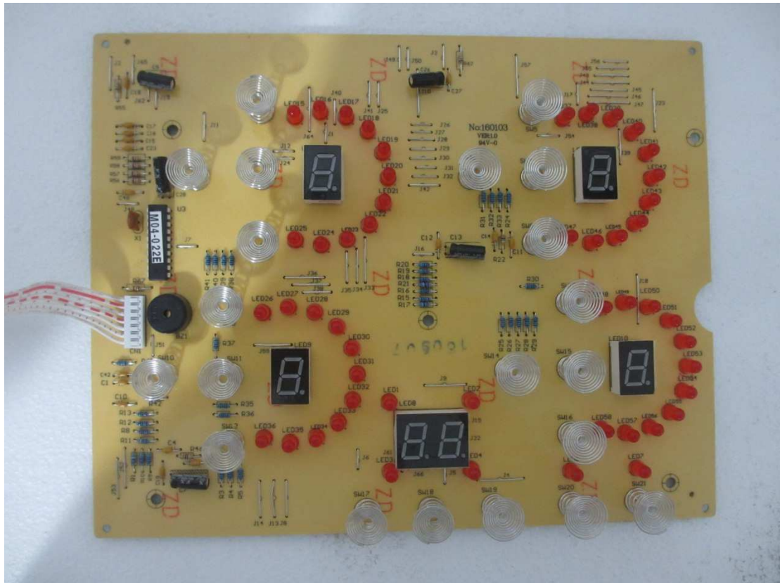
Control PCB:
