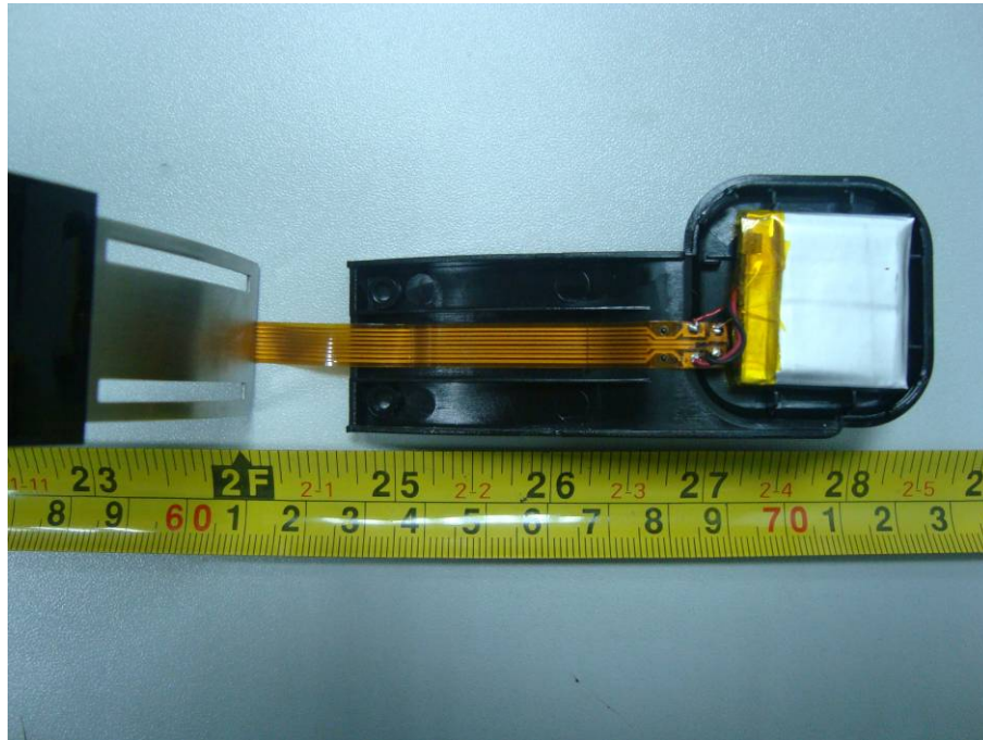
EUT – Left Side Cover off View
