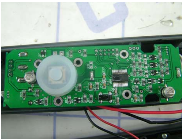
PCB2 layout
