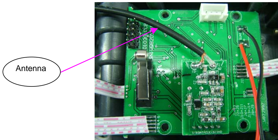
PCB1 solder
