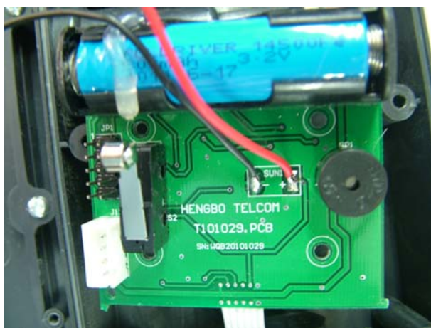
PCB3 solde
