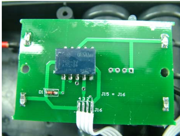
PCB2 solde
