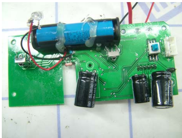
PCB1 solder
