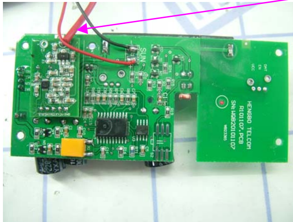
PCB1 layout
