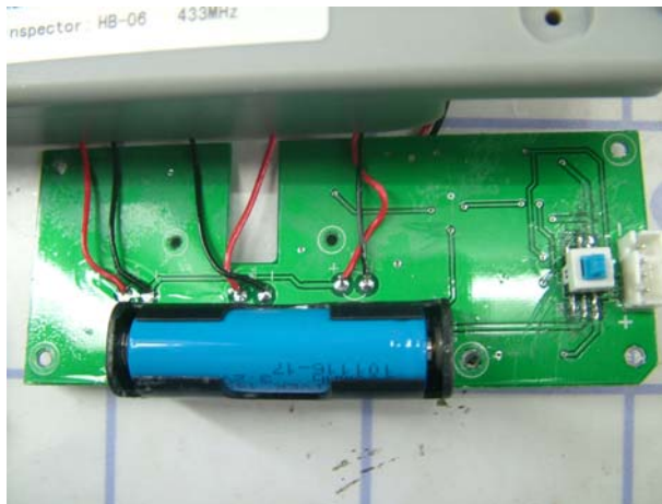
PCB2 solder
