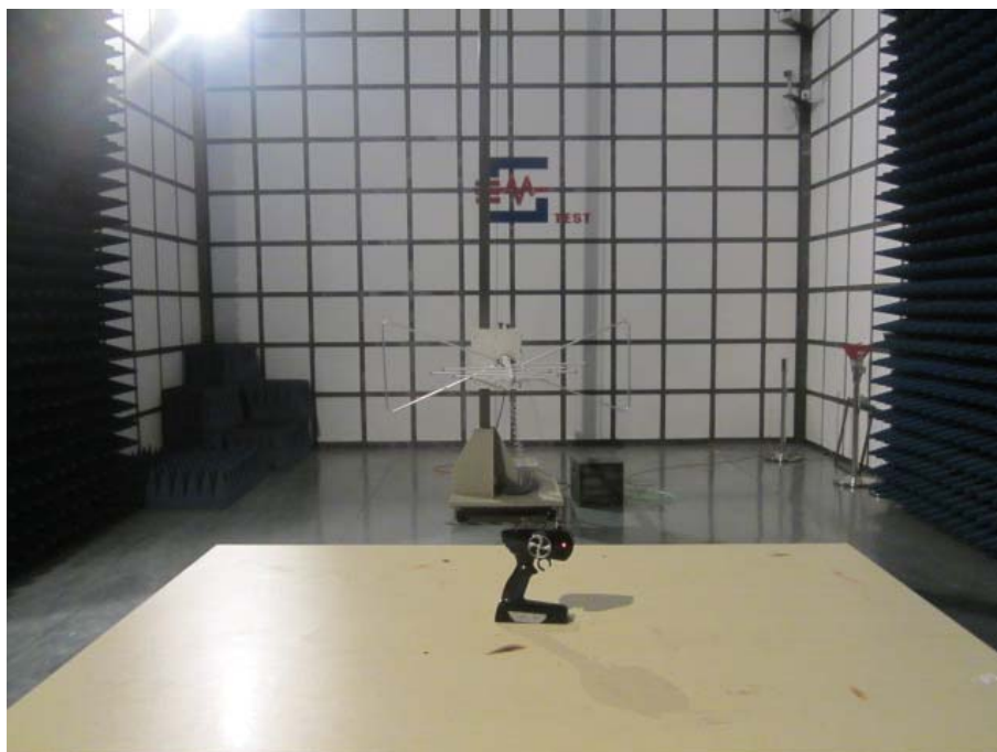
Radiated Emission Test Setup (30MHz to 1GHz)
