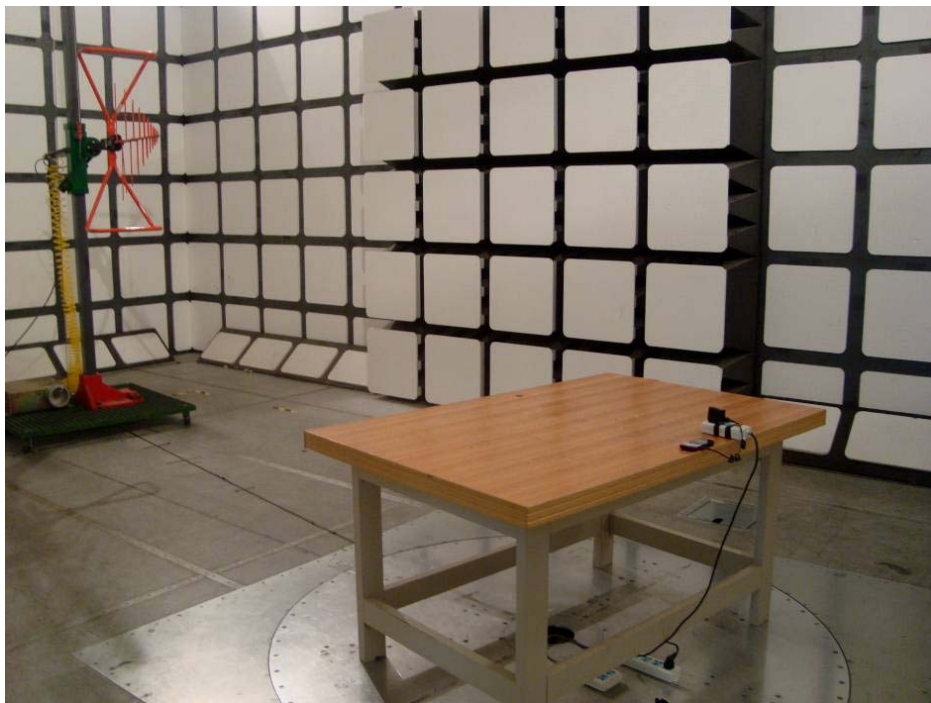
Radiated Emissions - Rear View (Adapter charging)
