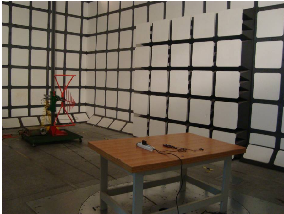
Radiated Emissions - Front View (Adapter charging & media playing)
