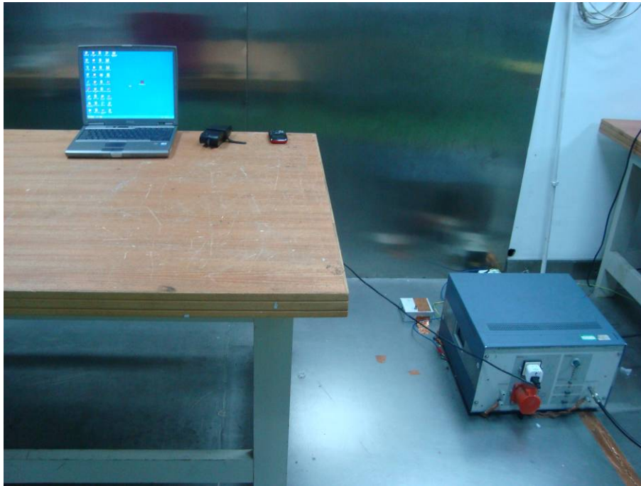
Conduction Emissions - Side View (PC charging)
