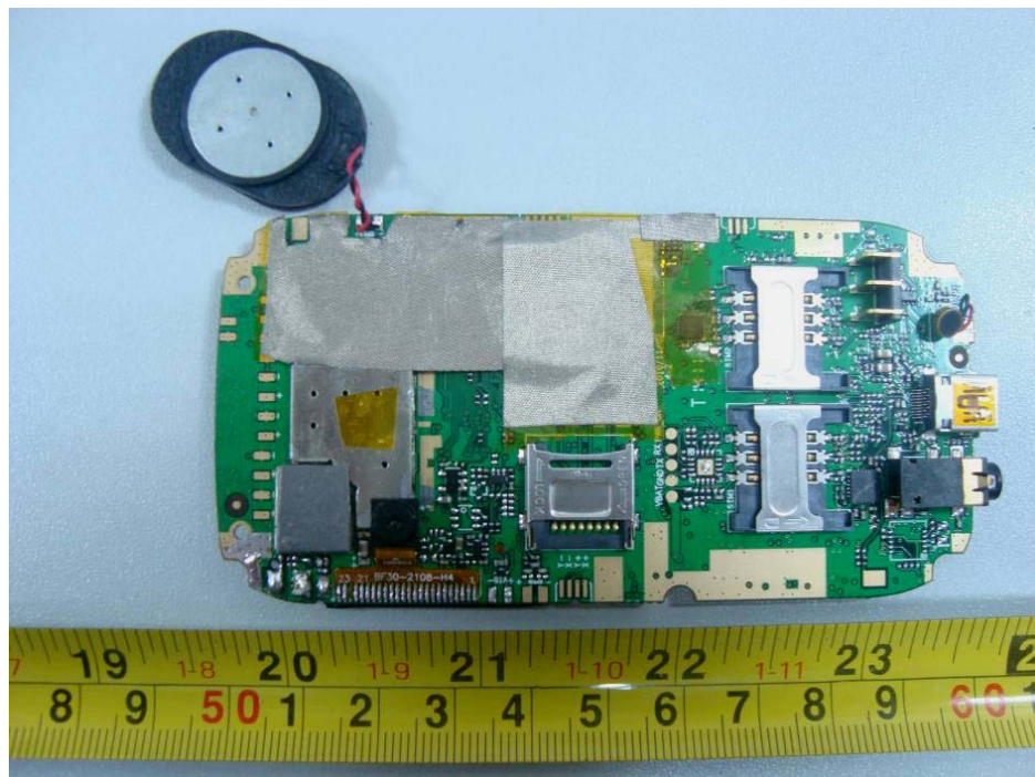
EUT – Main Board without Antenna Top View
