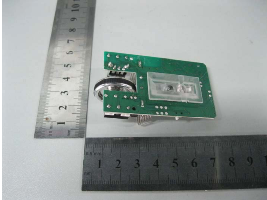
Figure 5 PCB of the EUT- PCB Face View
