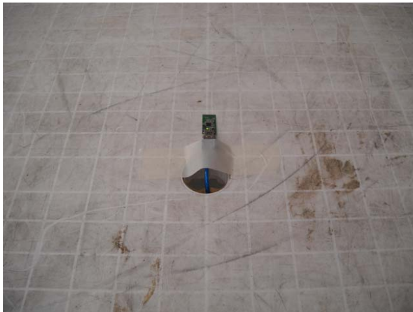
Photograph No.7 Setup for radiated emission measurements at the OATS, EUT close view
