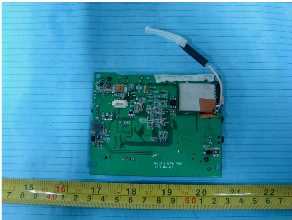
EUT – Main Board without LCD Shielding off Bottom View
