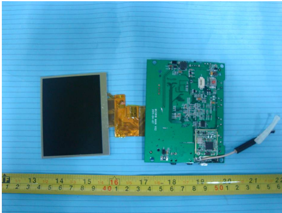
EUT – Main Board with LCD Shielding off Bottom View
