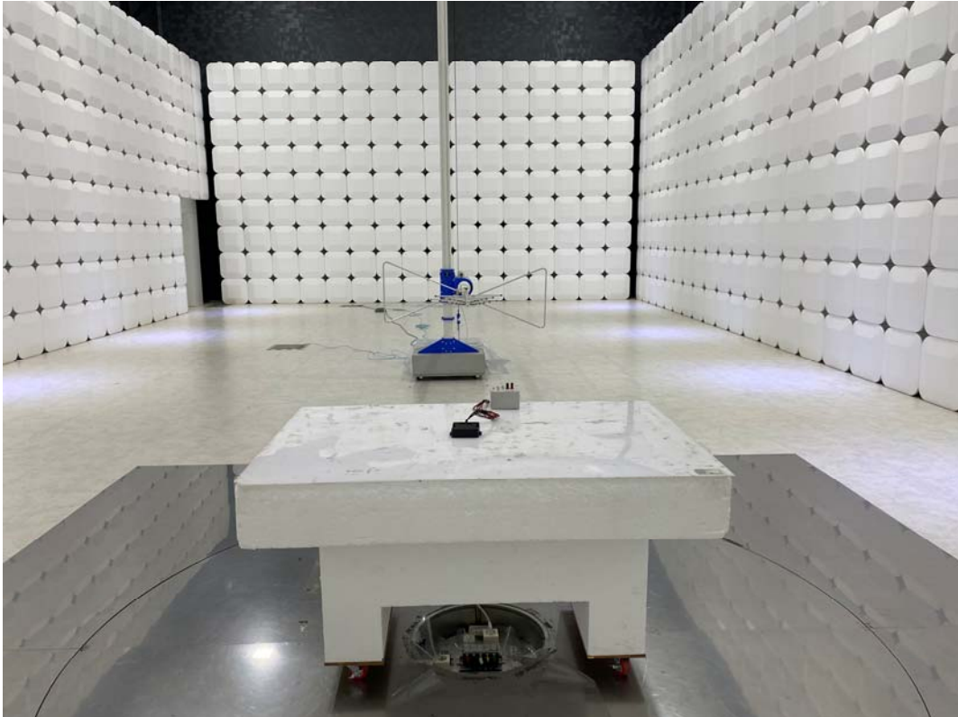
Radiated emission test (30 MHz to 1 GHz) – Front view
