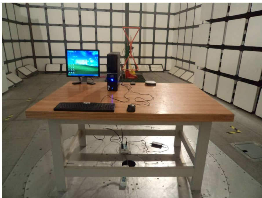
Radiated Emissions for Downloading Mode - Front View
