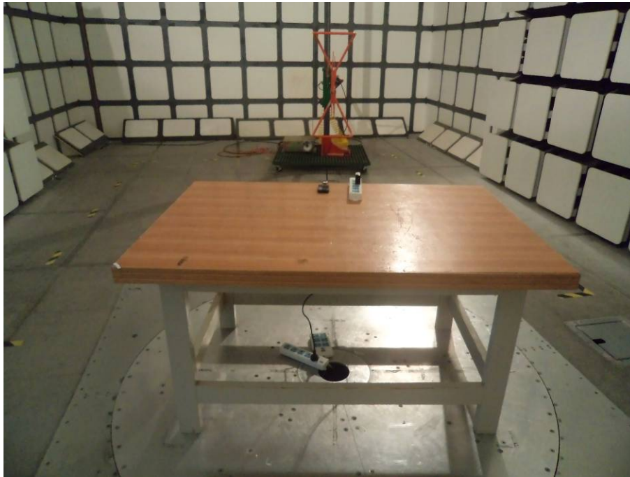
Radiated Emissions for Charging Mode - Front View
