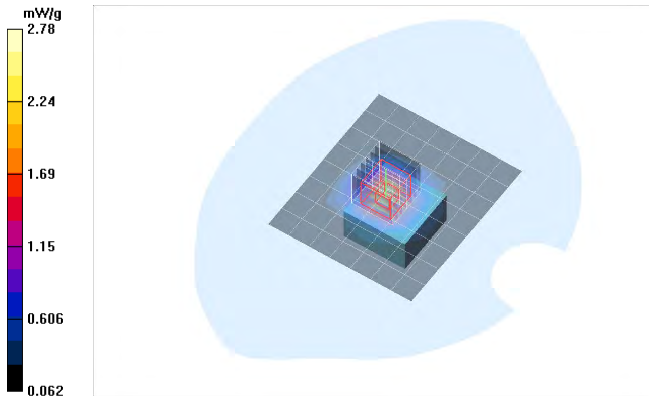
Plot. 3: SAR distribution plot for Smart Tag Location QUAD from buddi Limited, WCDMA 2, channel 9262, body position, 0mm distance, Configuration 1.
