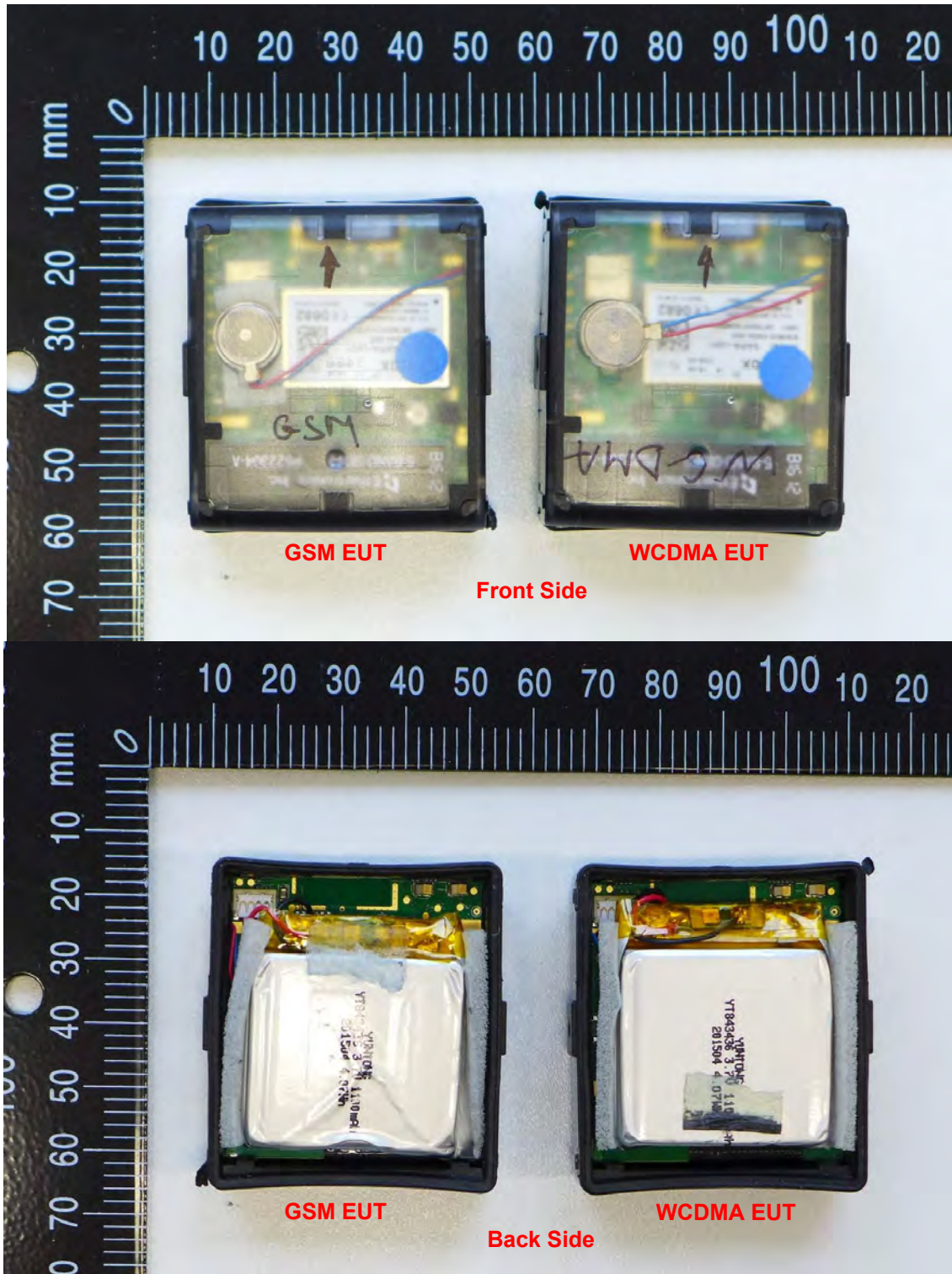
Pic. 2: Front and back views of the EUT without housing.
