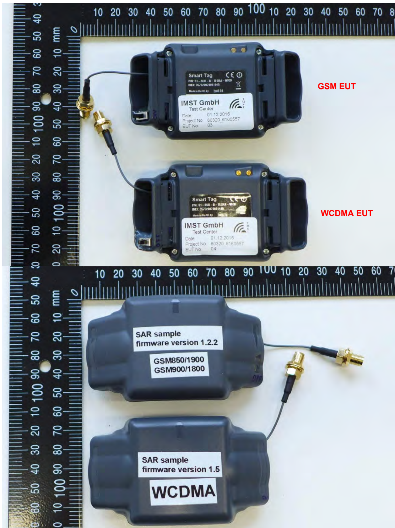
Pic. 5: Pictures of the conducted sample for GSM and WCDMA bands – back and front sides
