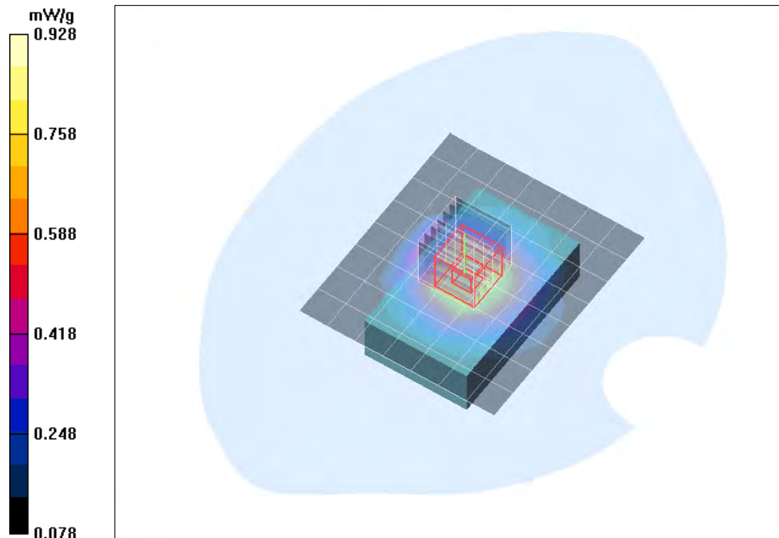
Plot 1: SAR distribution plot for Smart Tag Location QUAD from buddi Limited, GPRS 850 4TX, channel 128, body position, 0mm distance, Configuration 1.
