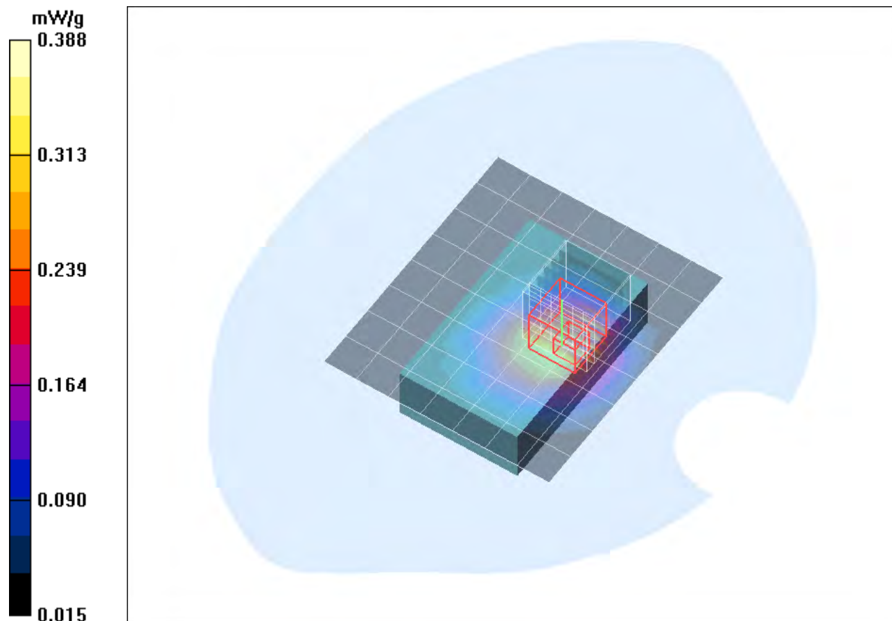
Plot. 4: SAR distribution plot for Smart Tag Location QUAD from buddi Limited, WCDMA 5, channel 4183, body position, 0mm distance, Configuration 2.
