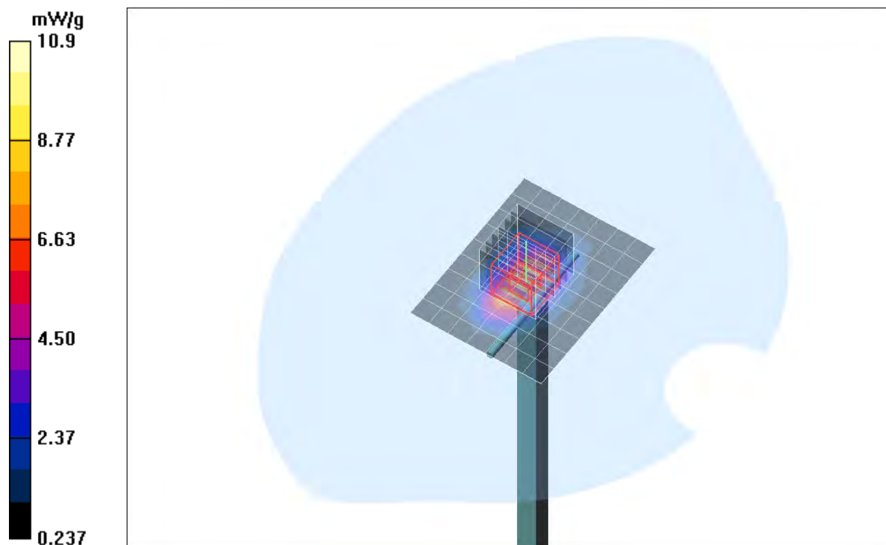
Plot. 5: System verification measurement 1900 MHz Body (GPRS 1900, WCDMA 2, December 06, 2016)
