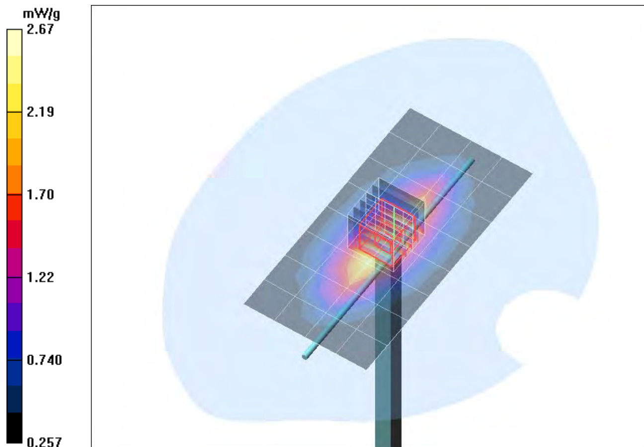
Plot. 6: System verification measurement 835 MHz Body (GPRS 850, WCDMA 5, December 08, 2016)
