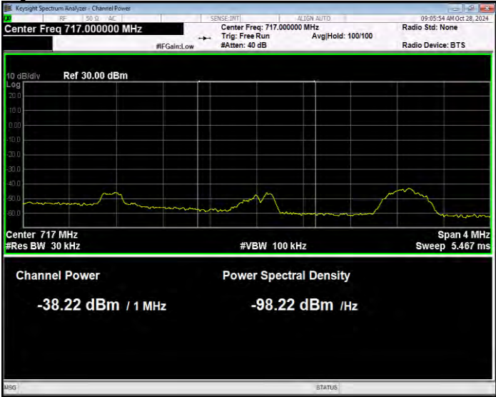
Band12 QPSK BW=3MHz Channel=23165 RB Size=1 Position=#0 Normal
