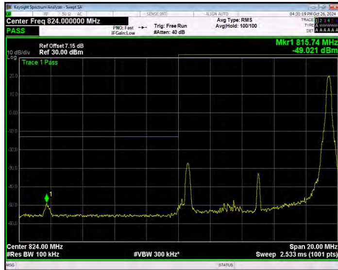
Band5 16QAM BW=10MHz Channel=20450 RB Size=27 Position=#0 Extended
