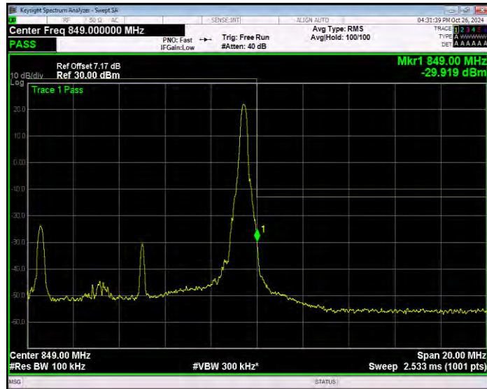
Band5 QPSK BW=10MHz Channel=20600 RB Size=50 Position=#0 Extended
