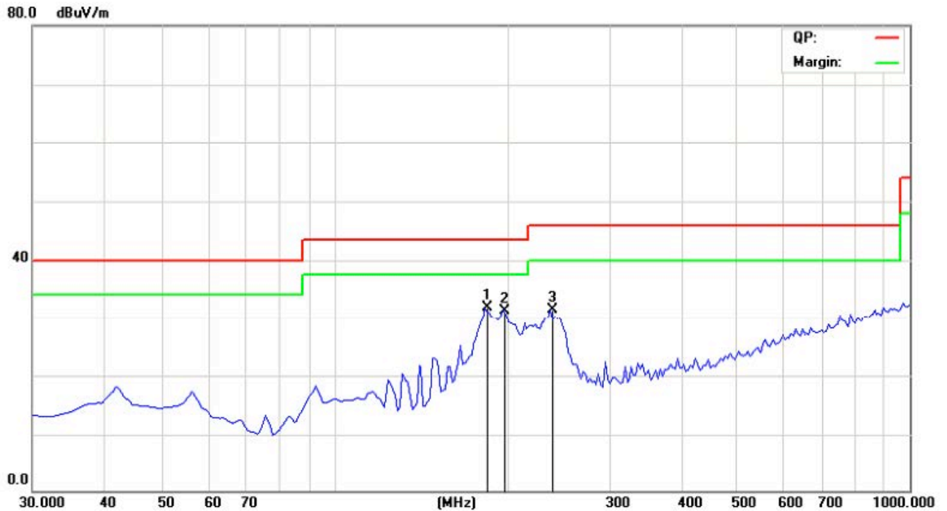
Test Result of Radiated Emission Test-Vertical-3m
