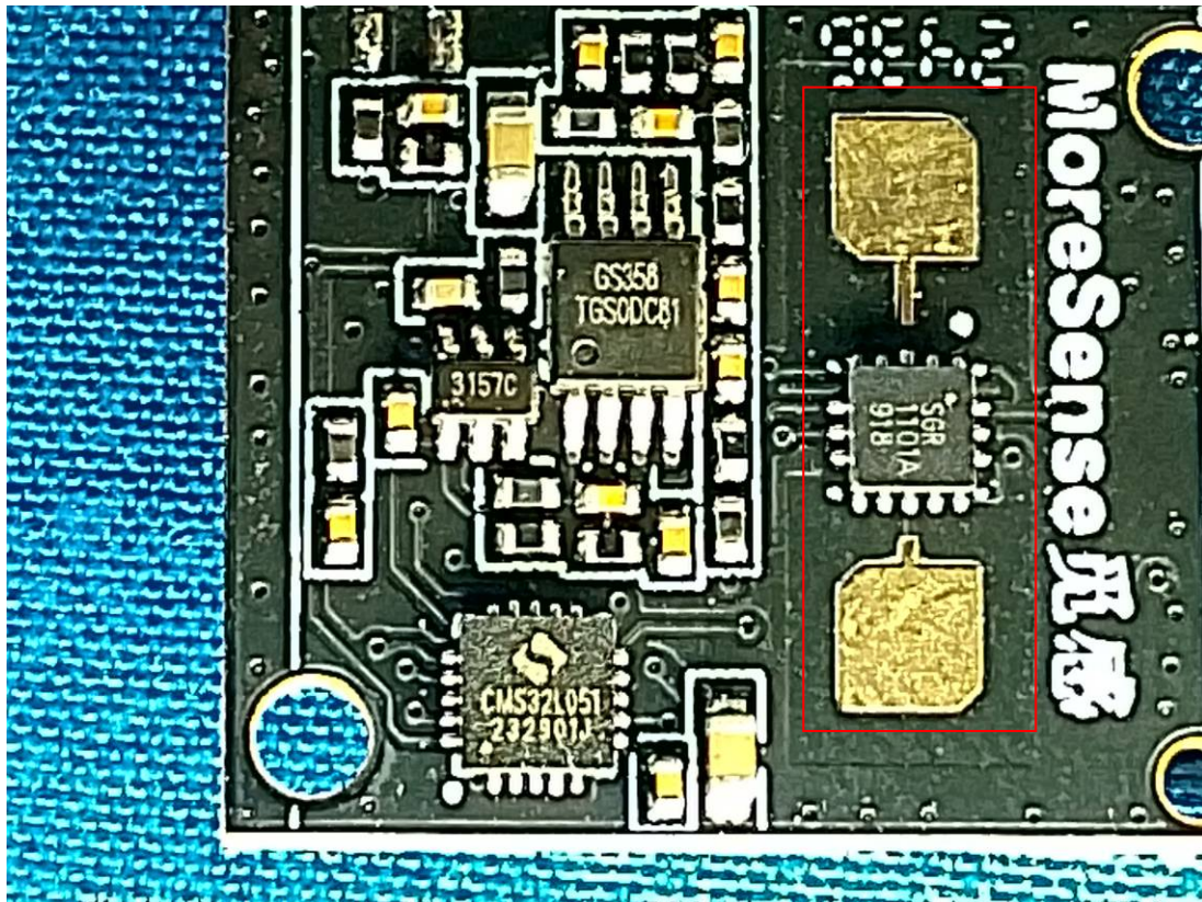
Radar Chip+Radar Antenna 1
