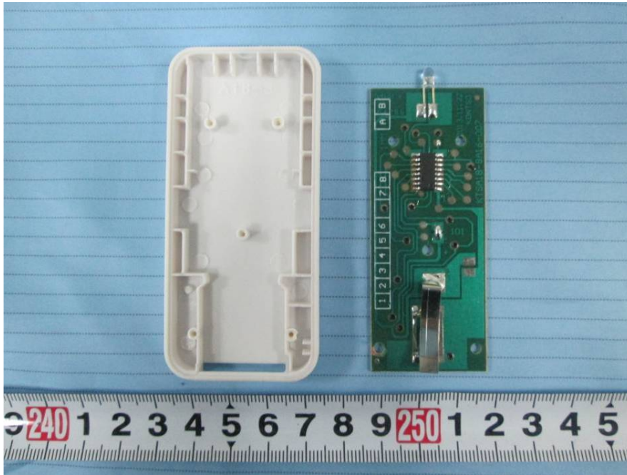
EUT – Cover off View 3 (Remote-controller)
