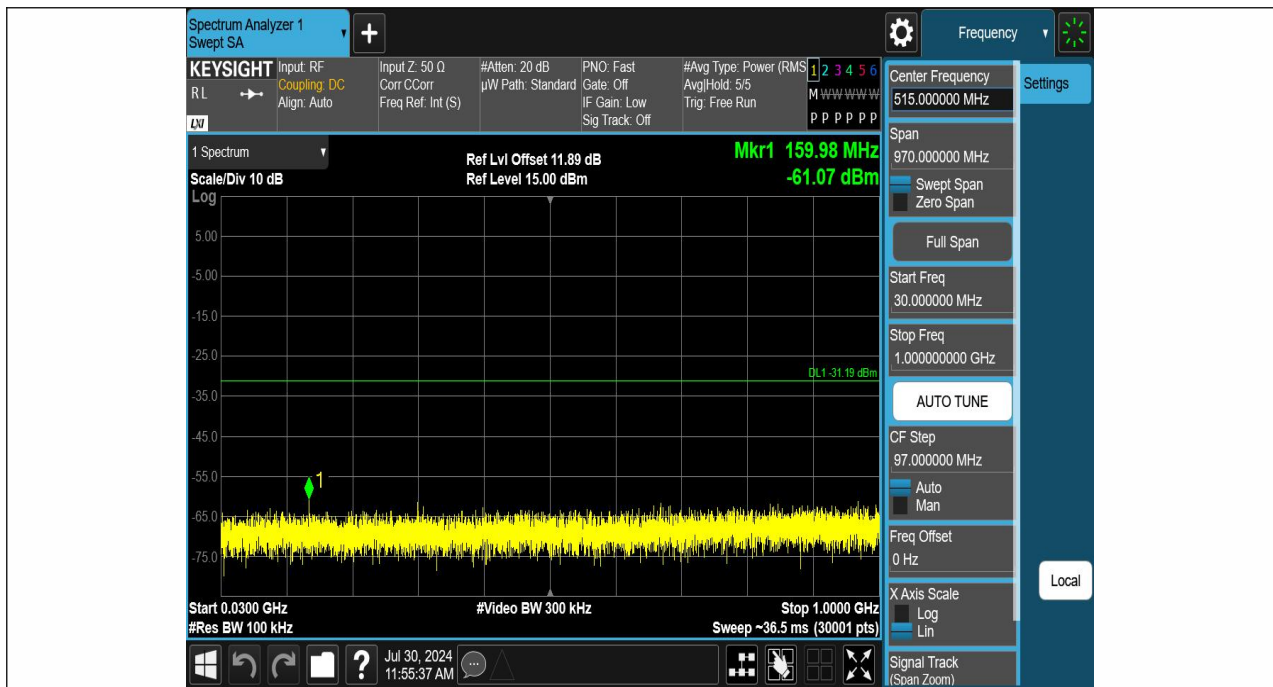
11N20SISO-Ant1-2437-30~1000-PASS
