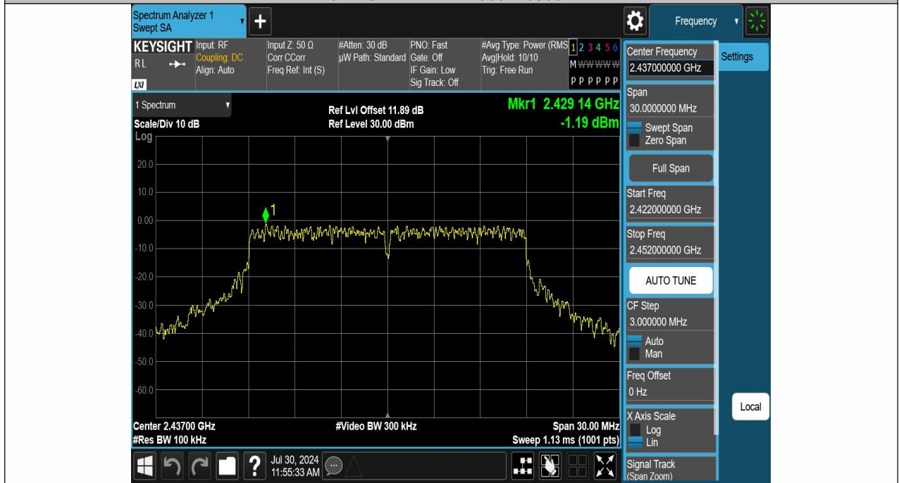
11N20SISO-Ant1-2437-0~Reference-PASS
