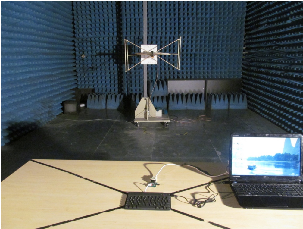
FCC RADIATED EMISSION TEST SETUP (Continuous TX)
