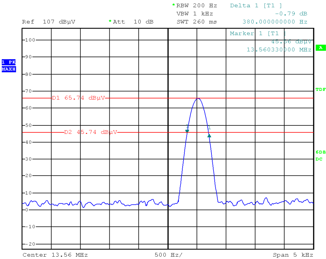
20dB Bandwidth
