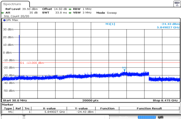
3MHz_High_QPSK_15@0 -24.43 dBm
