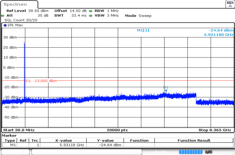
1.4MHz_Mid_QPSK_6@0 -24.64 dBm
