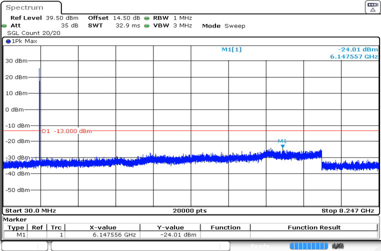
1.4MHz_Low_QPSK_6@0 -24.01 dBm
