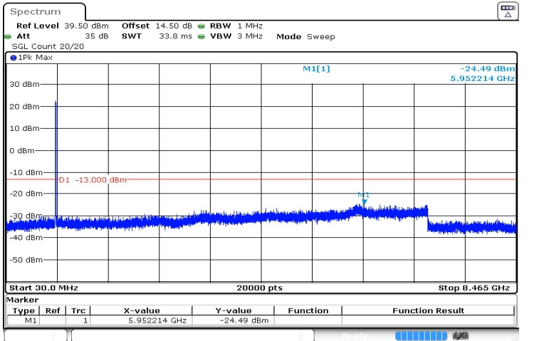
5MHz_High_QPSK_25@0 -24.49 dBm
