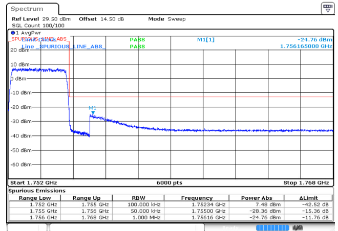
3MHz_High_16QAM_15@0 -24.76dBm
