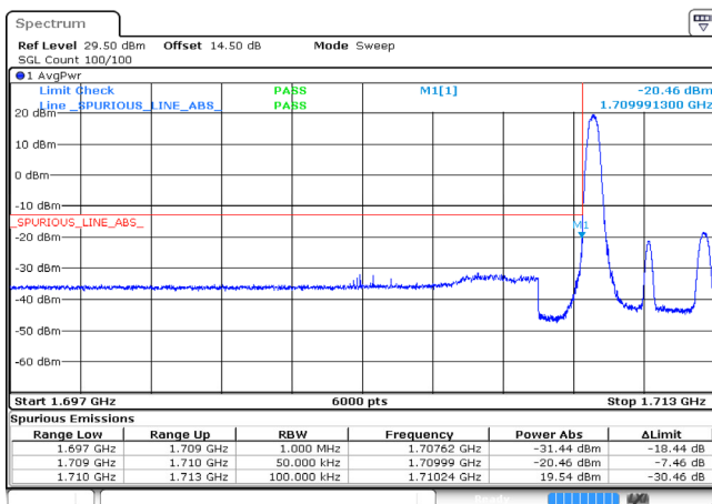
3MHz_Low_16QAM_1@0 -20.46dBm
