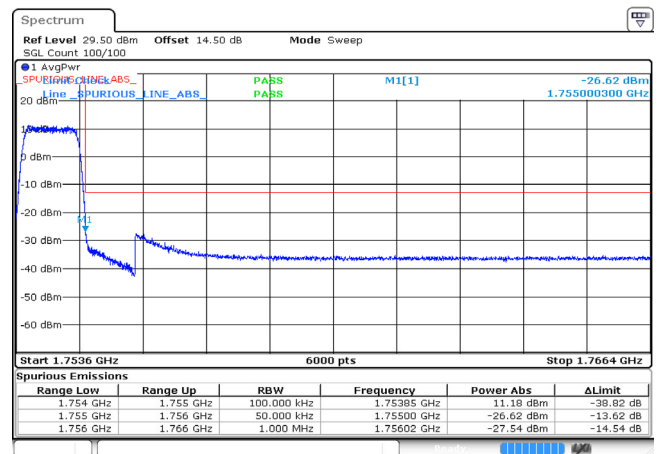
1.4MHz_High_16QAM_6@0 -26.62dBm
