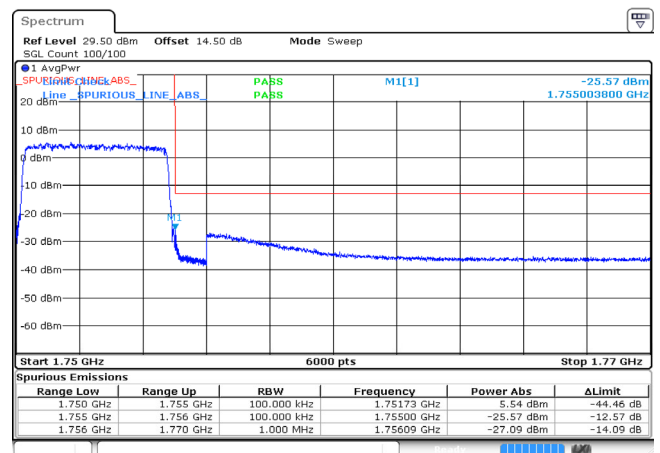
5MHz_High_16QAM_25@0 -25.57dBm
