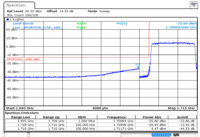
5MHz_Low_16QAM_25@0 -25.60dBm
