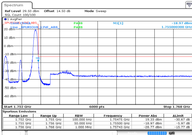
3MHz_High_16QAM_1@14 -18.97dBm
