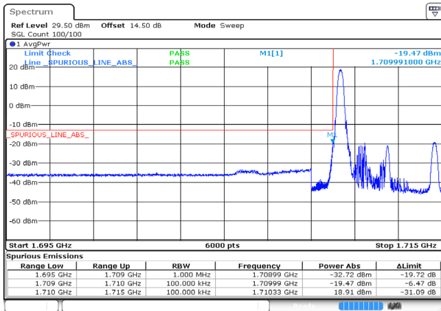
5MHz_Low_16QAM_1@0 -19.47dBm
