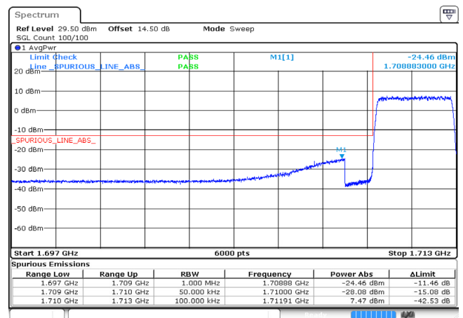
3MHz_Low_16QAM_15@0 -24.46dBm
