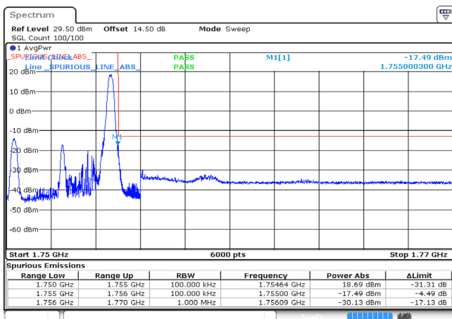
5MHz_High_16QAM_1@24 -17.49dBm
