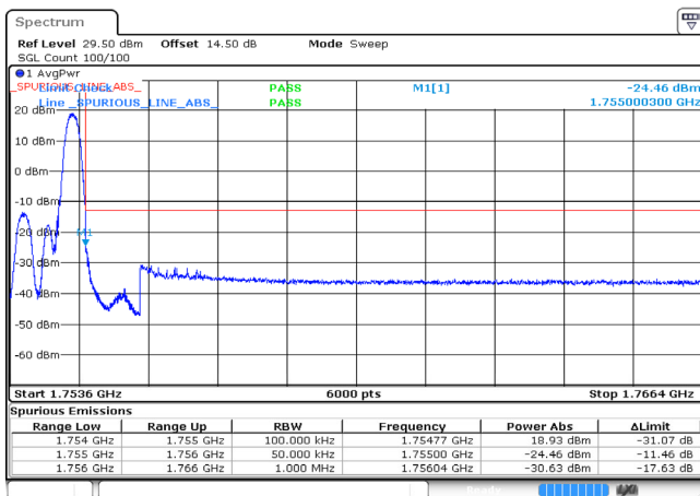
1.4MHz_High_16QAM_1@5 -24.46dBm
