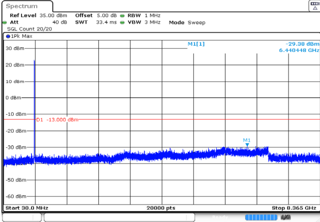
3MHz_Middle_QPSK_15@0 -29.38dBm
