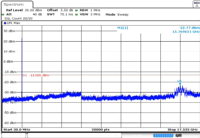
3MHz_High_QPSK_15@0 -22.77dBm
