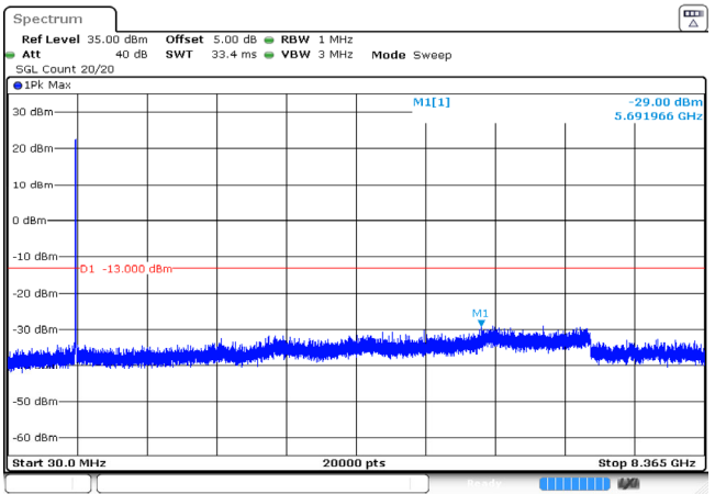
5MHz_Middle_QPSK_25@0 -29.00dBm
