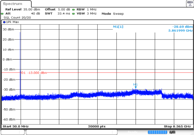
3MHz_Middle_QPSK_1@0 -28.69dBm
