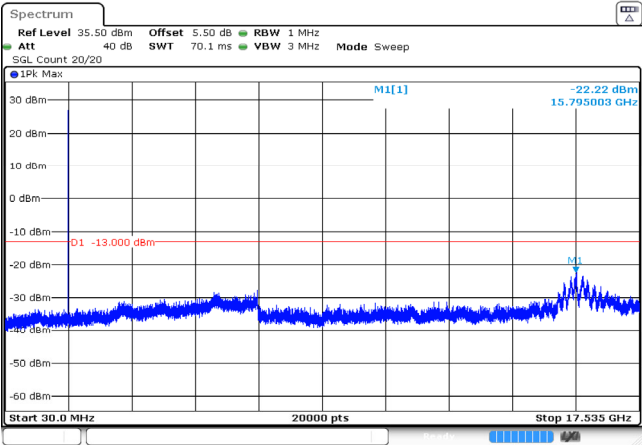
3MHz_High_QPSK_1@0 -22.22dBm
