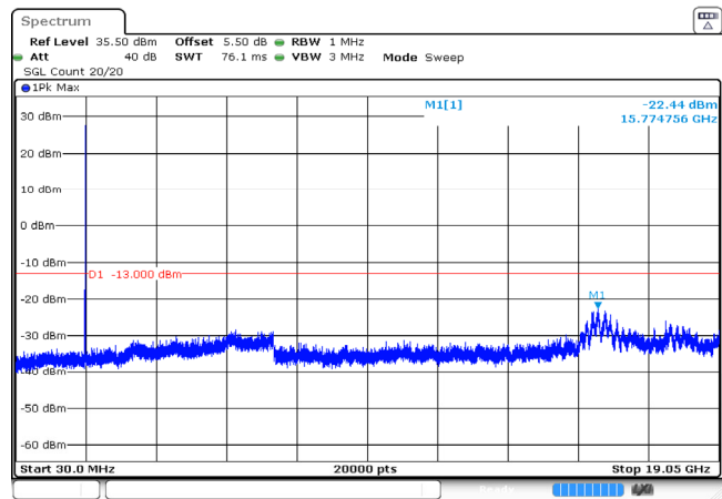
10MHz_High_QPSK_1@0 -22.44dBm
