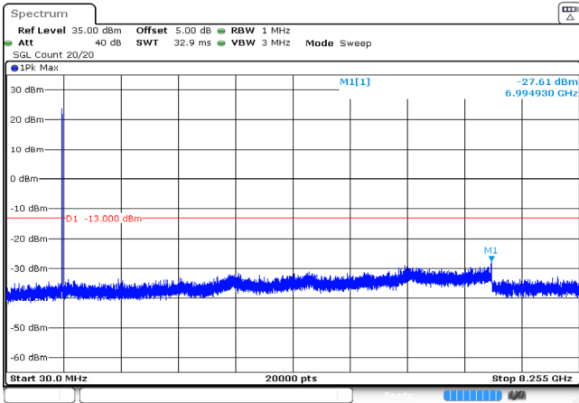
3MHz_Low_QPSK_15@0 -27.61dBm
