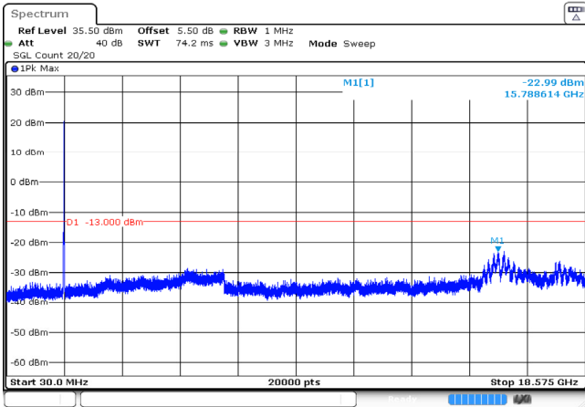
15MHz_Low_QPSK_75@0 -22.99dBm
