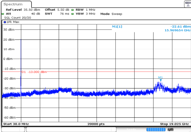
15MHz_High_QPSK_75@0 -22.61dBm
