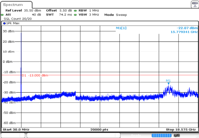
15MHz_Low_QPSK_1@0 -22.07dBm
