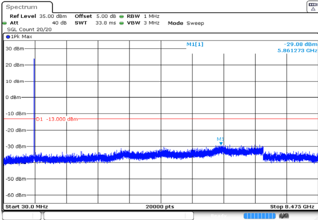
3MHz_High_QPSK_15@0 -29.08dBm
