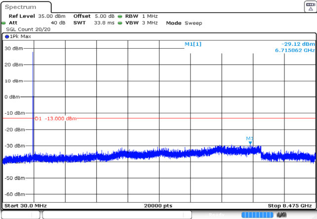
3MHz_High_QPSK_1@0 -29.12dBm
