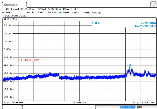
10MHz_High_QPSK_50@0 -22.97dBm
