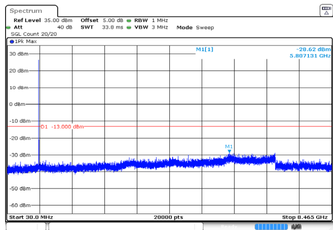
5MHz_High_QPSK_1@0 -28.62dBm
