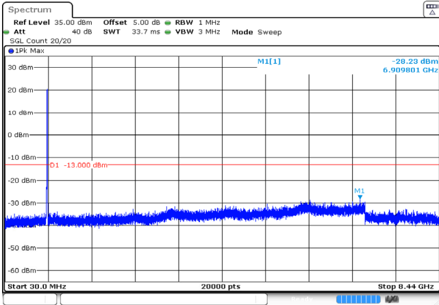
10MHz_High_QPSK_50@0 -28.23dBm
