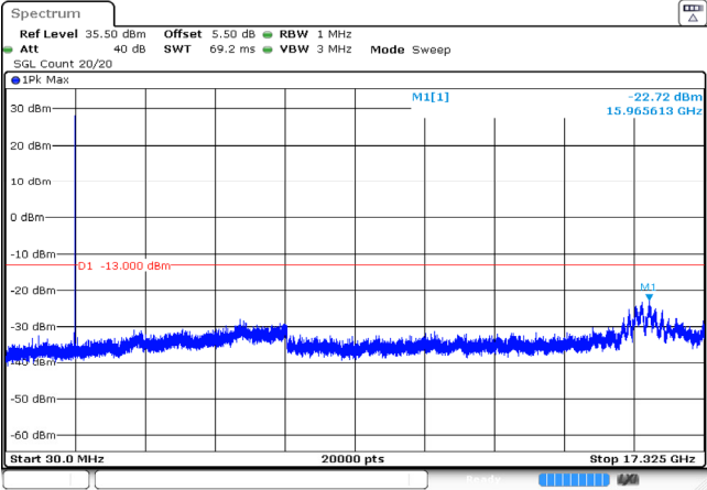
3MHz_Middle_QPSK_1@0 -22.72dBm
