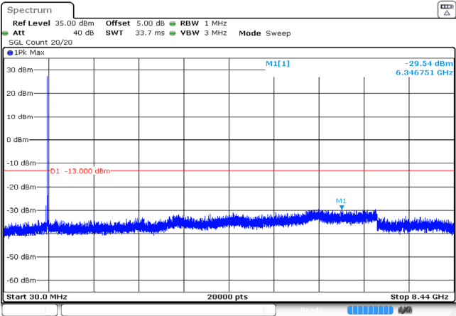
10MHz_High_QPSK_1@0 -29.54dBm
