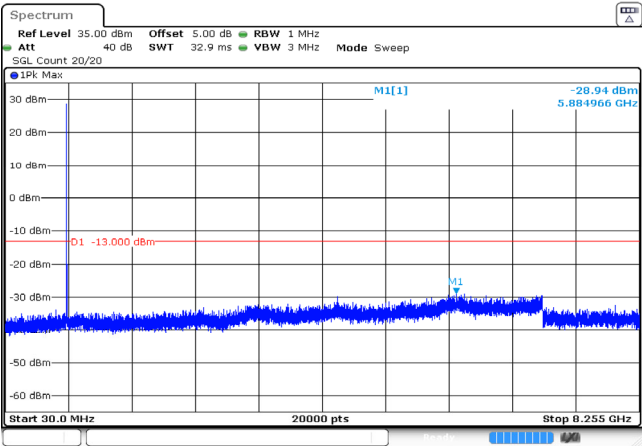
3MHz_Low_QPSK_1@0 -28.94dBm
