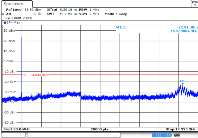
3MHz_Middle_QPSK_15@0 -22.91dBm
