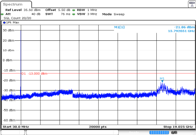
15MHz_High_QPSK_1@0 -21.86dBm
