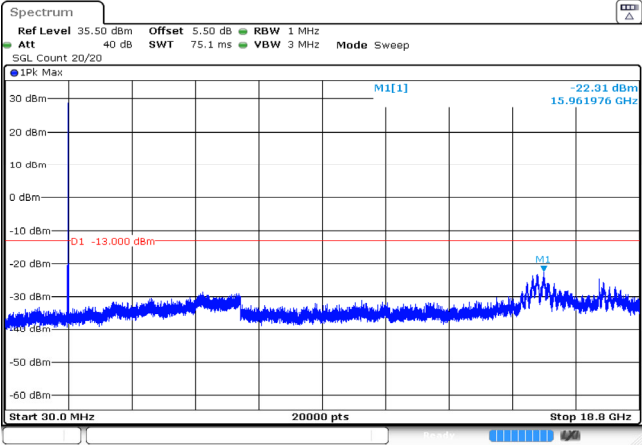
15MHz_Middle_QPSK_1@0 -22.31dBm
