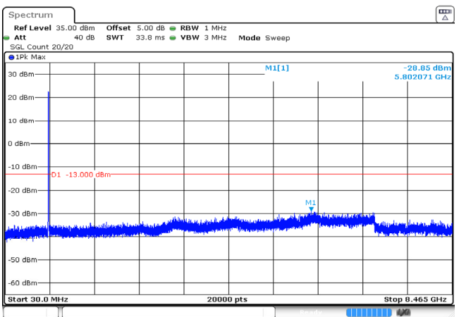
5MHz_High_QPSK_25@0 -28.85dBm
