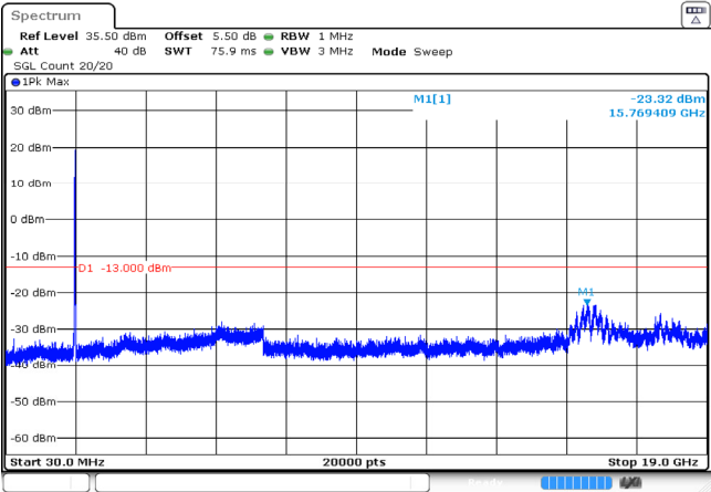
20MHz_High_QPSK_100@0 -23.32dBm
