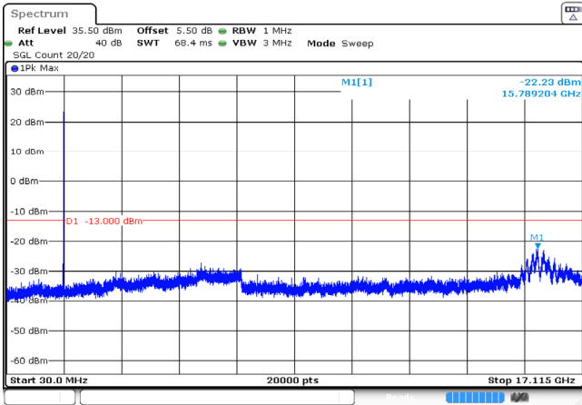
3MHz_Low_QPSK_15@0 -22.23dBm
