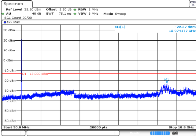
15MHz_Middle_QPSK_75@0 -22.57dBm
