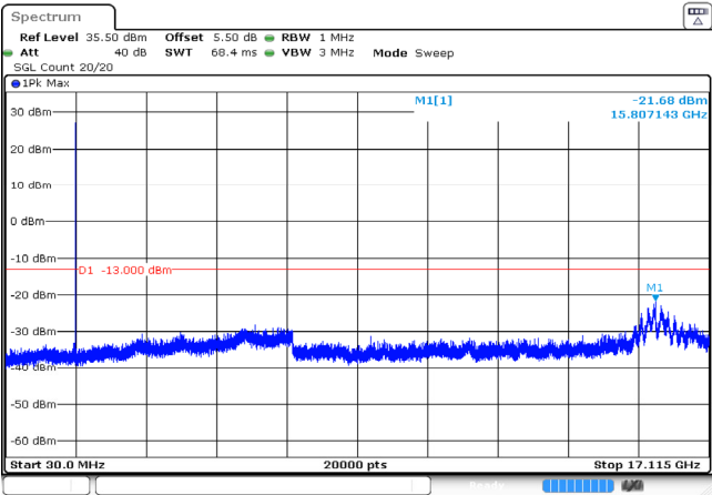
3MHz_Low_QPSK_1@0 -21.68dBm
