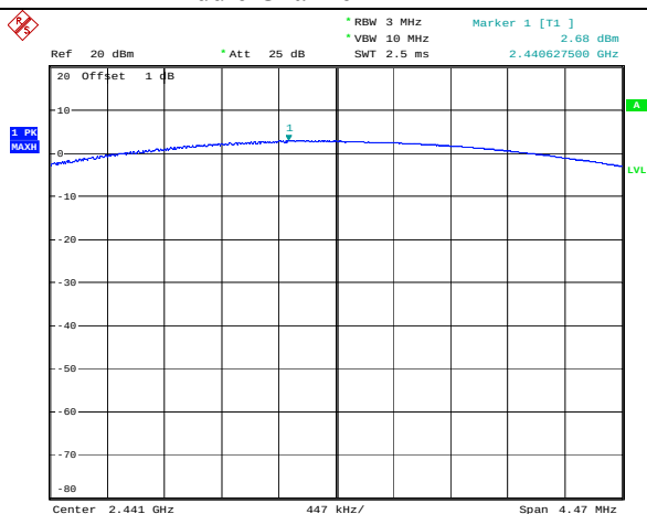
Middle Channel 2441MHz
