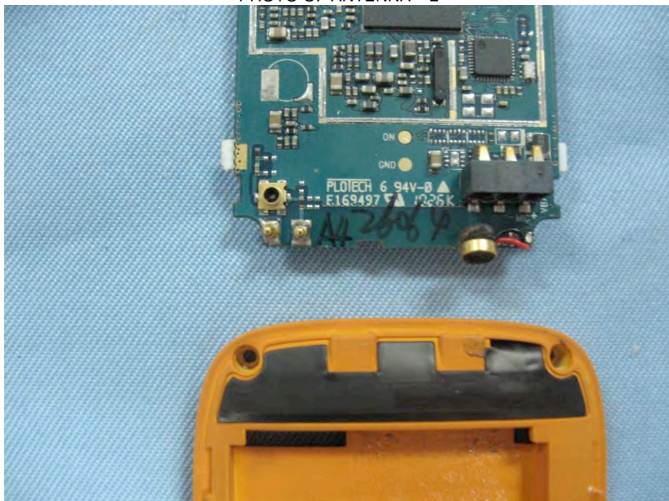
PHOTO OF ANTENNA – 2
