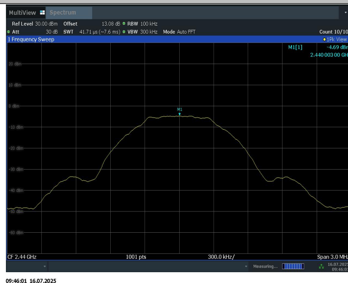
BLE_1M_2440_0~Reference
